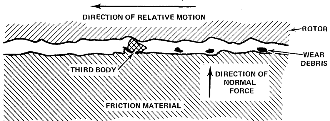
Figure 2-12 - Mechanism of Three-Body Abrasive Wear
