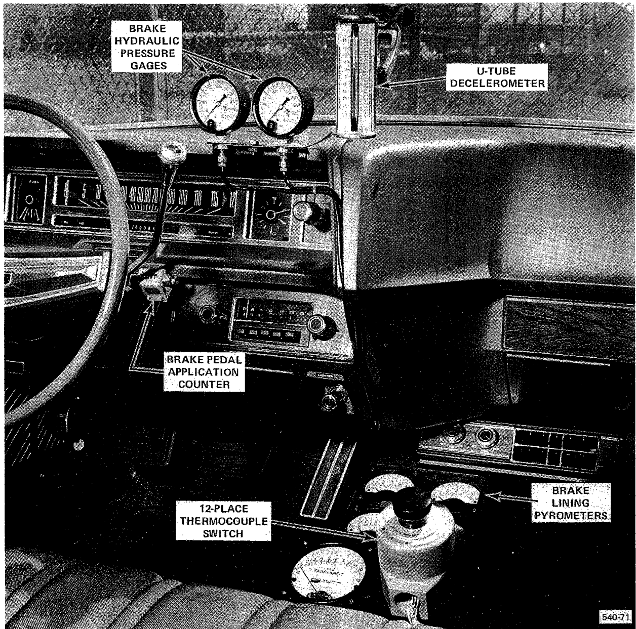
Figure 4-1 - Vehicle Instrumentation for Friction Material Testing
