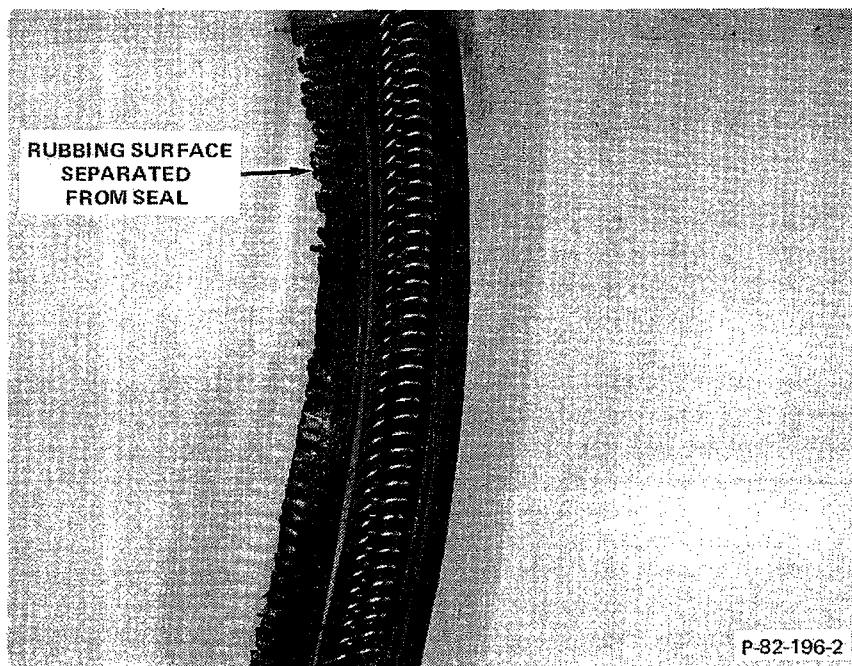
Figure 5-27 - Completely Worn Seal from MKII Rear Drum Brake Collector
