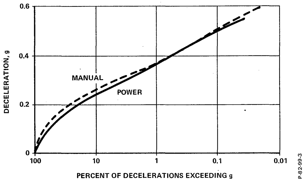
Figure 10-1 - Frequency Distribution of Braking Decelerations
