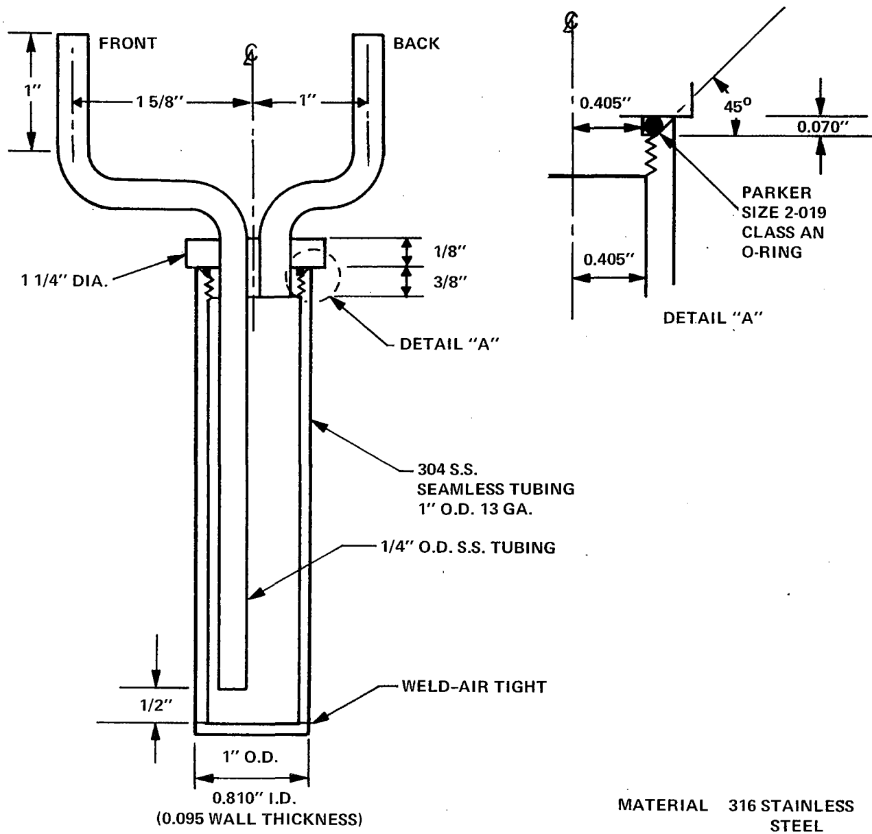
Figure 5-6 - Condensable-Gas Trap
