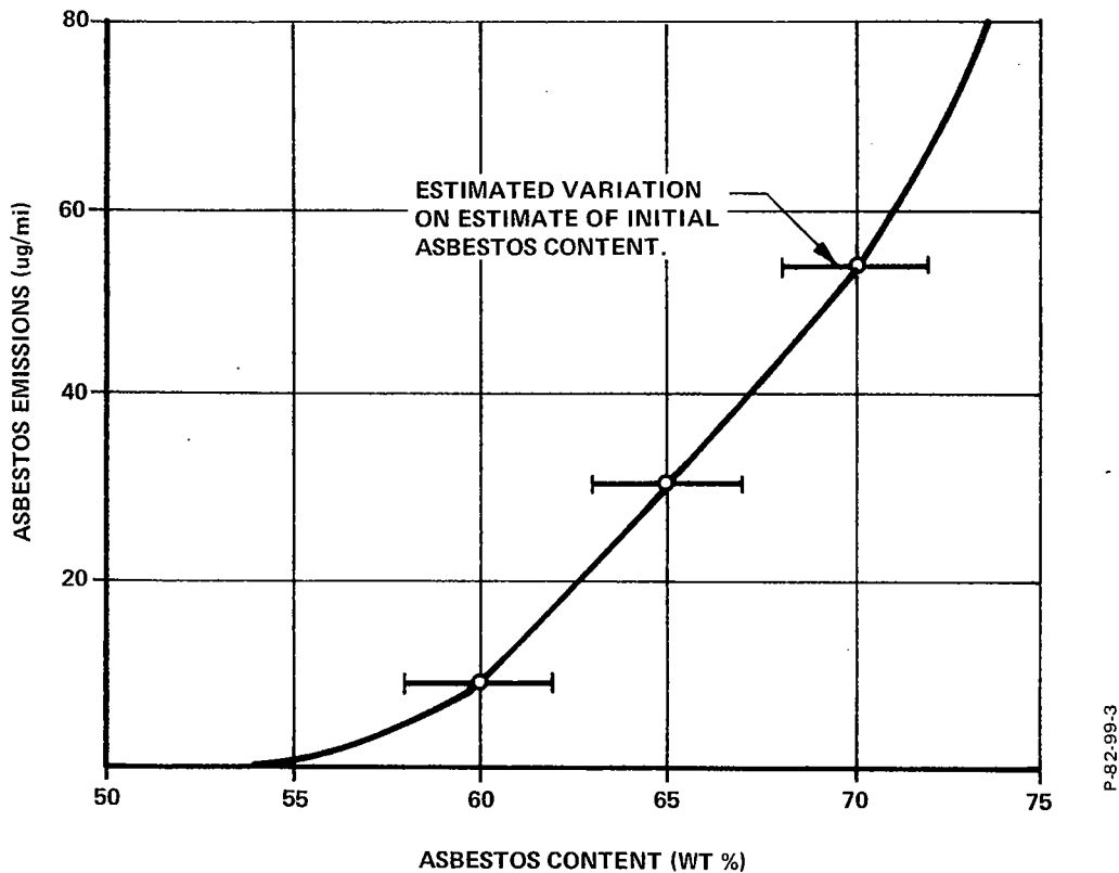
Figure 9-4 - Variation of Asbestos Emissions During Moderate Duty With Asbestos Content of Disc Pads
