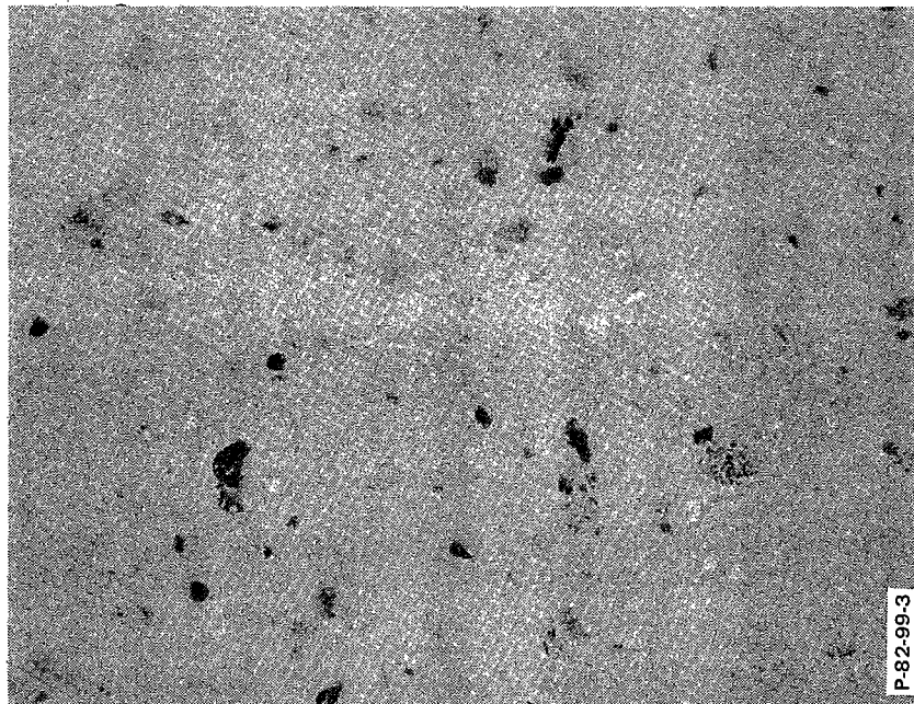
Figure 8-9 - Phase-Contrast Photomicrograph of Wear Debris - 400X
