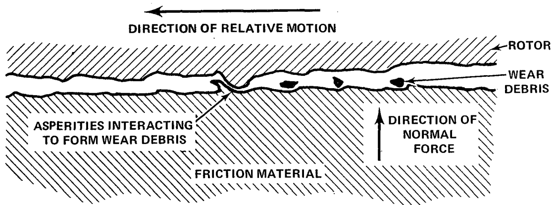
Figure 2-11 - Mechanism of Two-Body Abrasive Wear
