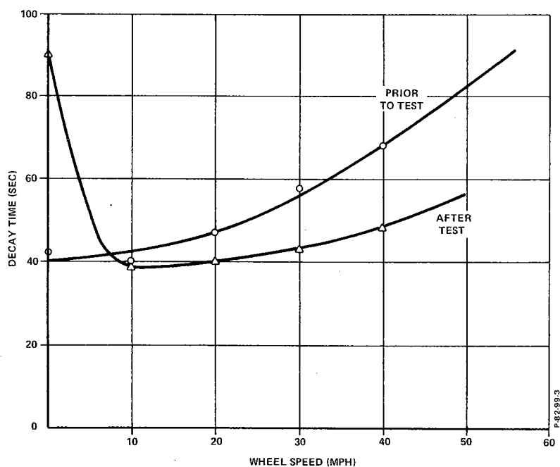
Figure 6-5 - Seal Leakage Rate Versus Speed Showing Differences Between New and Used Seal
