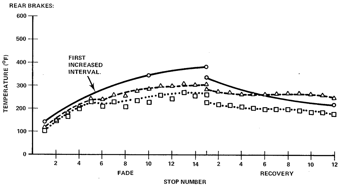
Figure 9-2 - Brake Temperature Data - Vehicle Test 1, 15-Stop Fade
