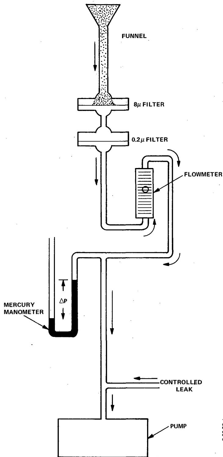
Figure B-1 - Sketch of Experimental Setup for Defining Filter Flow Characteristics of Nuclepore Membranes
