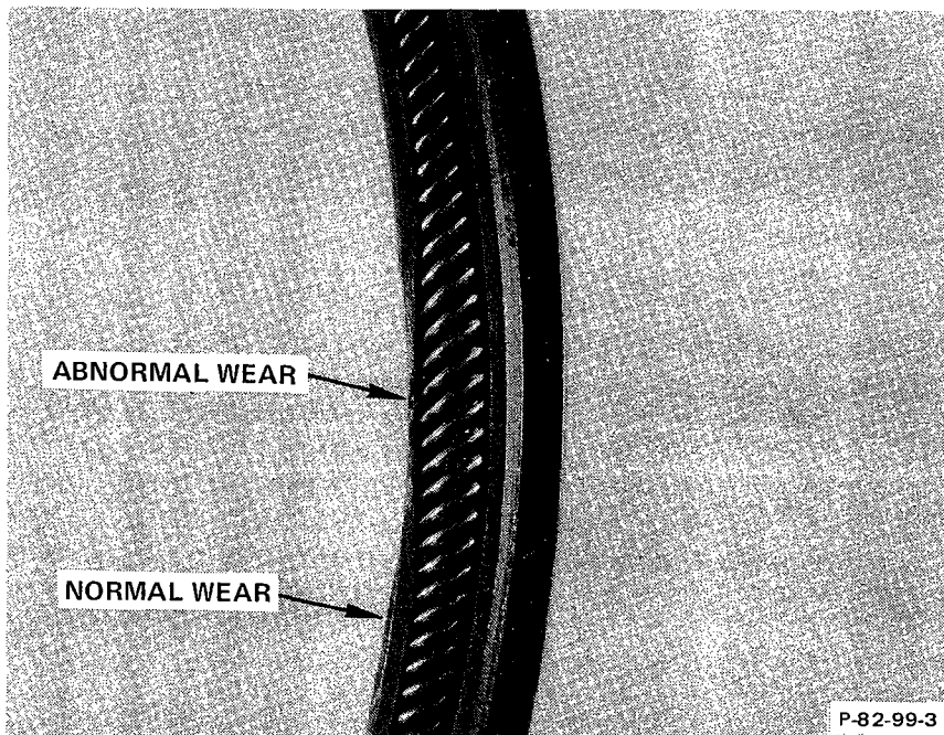
(b) Abnormal Wear to the Point of Imminent Seal Failure
