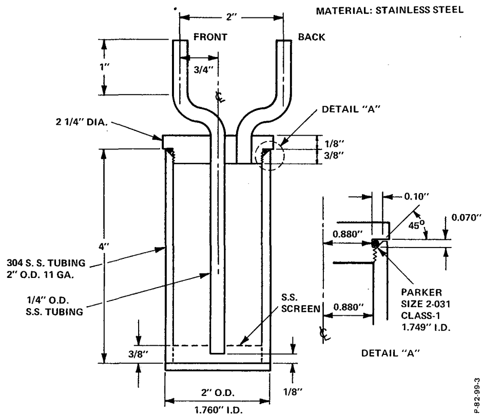
Figure 5-7 - Activated-Charcoal Gas Trap - Sectional View
