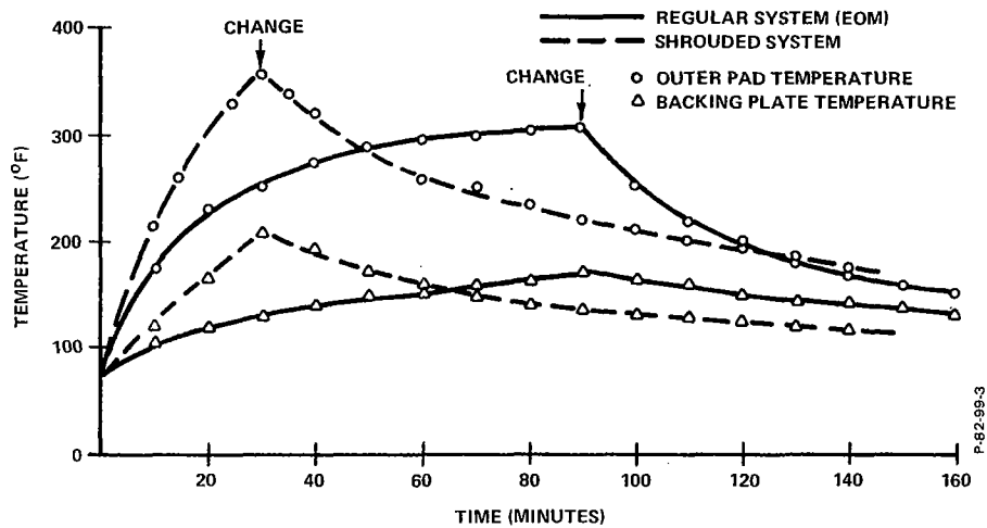
Figure 6-2 - Disc Brake Comparative Thermal Response Time (Static Air)
