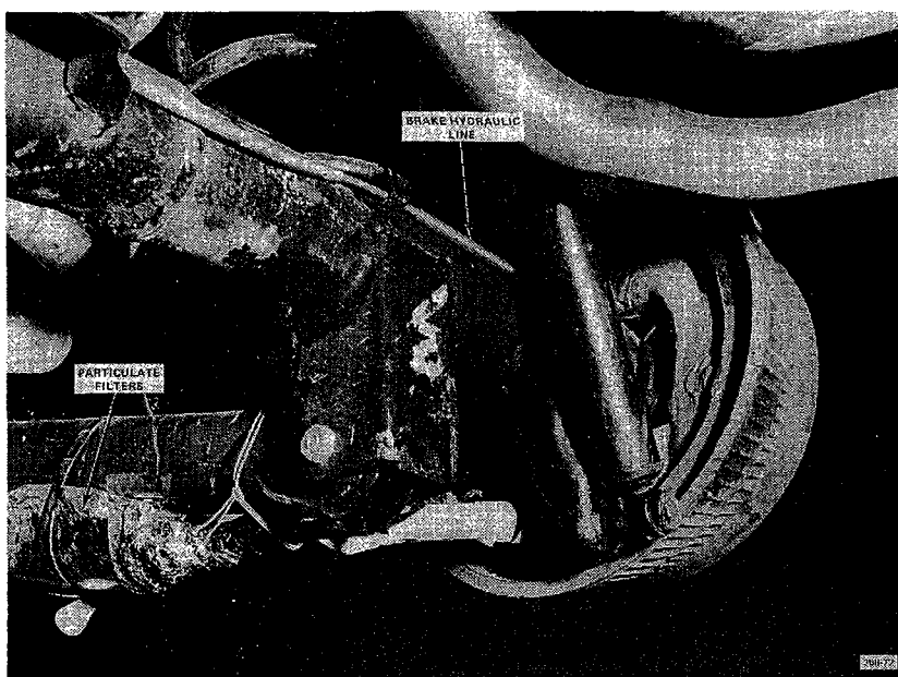
Figure 5-26 - Rear View of Rear Drum Brake Emissions Collector Showing Instrumentation
