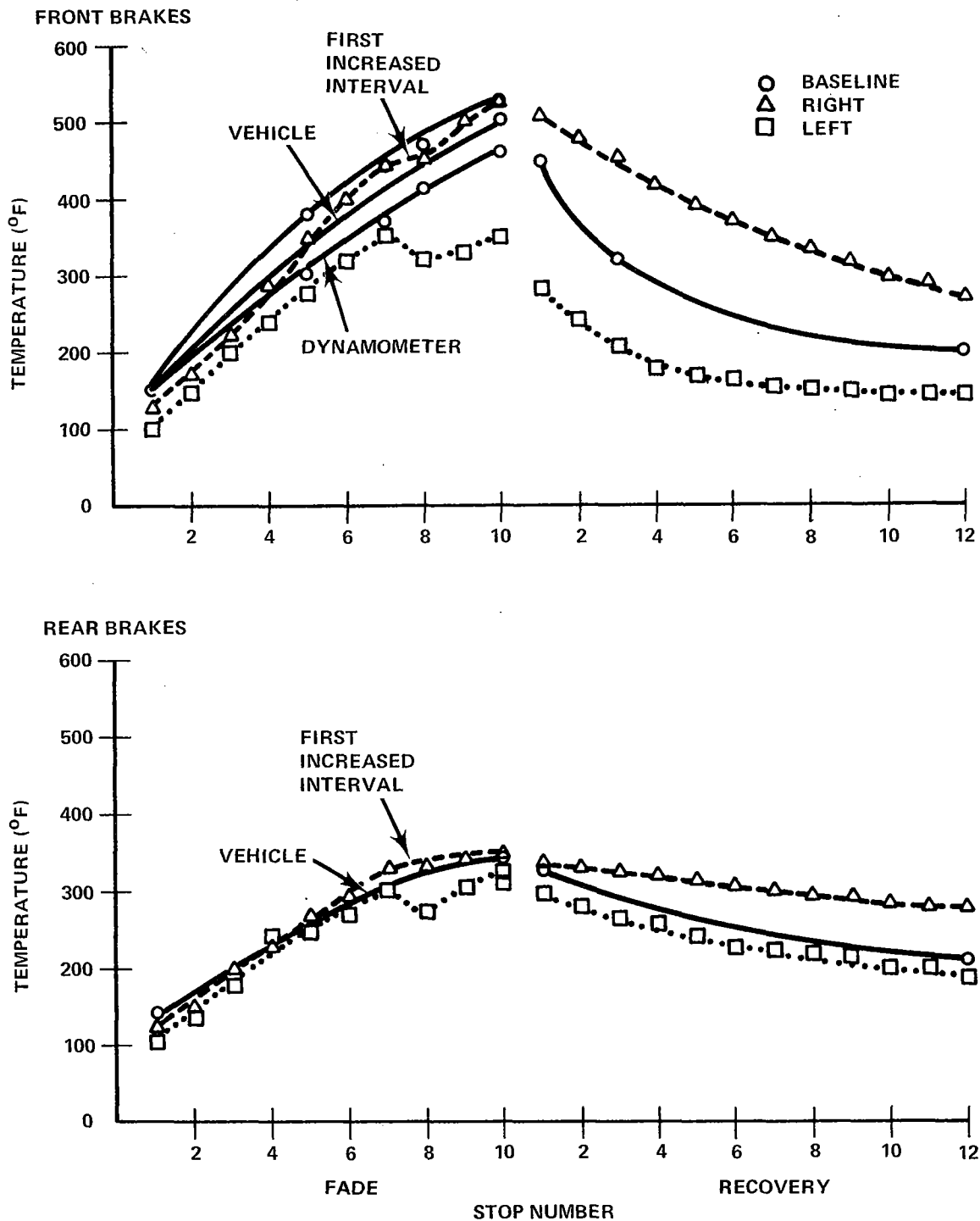
Figure 9-1 - Brake Temperature Data - Vehicle Test 1, 10-Stop Fade
