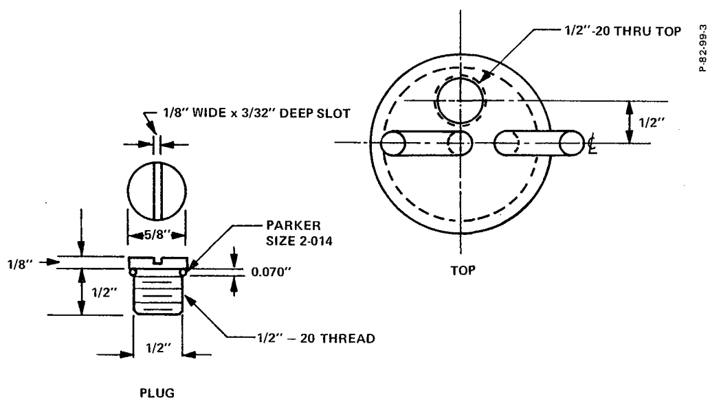
Figure 5-8 - Activated-Charcoal Gas Trap - Top View
