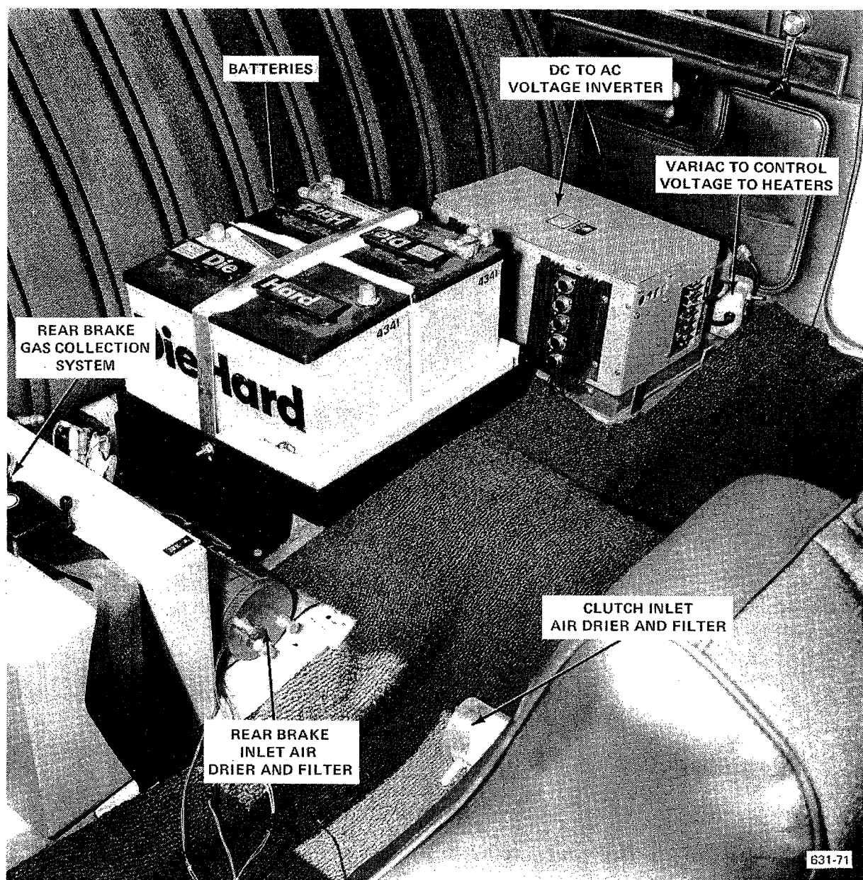
Figure 5-4 - Vehicle Instrumentation (Rear Seat Area)
