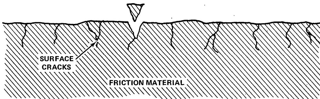
Figure 2-15 - Mechanism of Fatigue Wear
