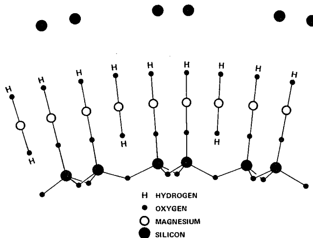
Figure 2-1 - Schematic Structure of Chrysotile Asbestos
