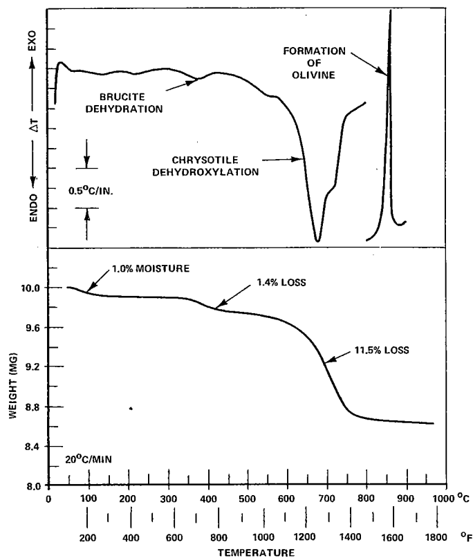
Figure 2-2 - DTA and TGA Thermograms for Chrysotile Asbestos (Bendix Data)
