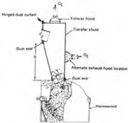
Hammermill Crusher
