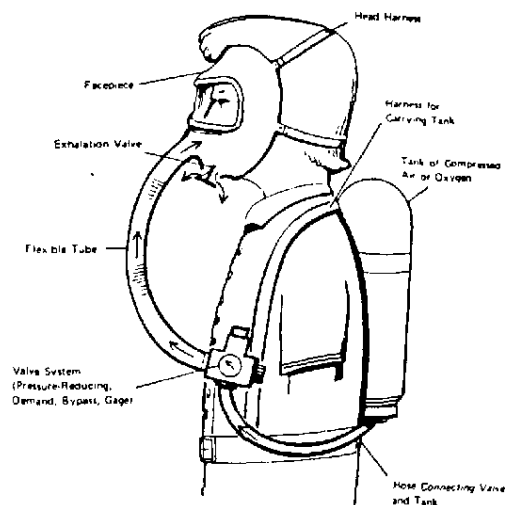
Fig. 5-30. Open-circuit SCBA.
