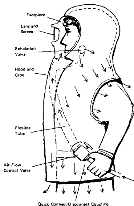
Fig. 5-7. Typical supplied-air blouse.
