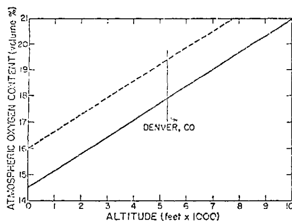
Fig. 4-2. The effect of altitude on the definition of oxygen deficient atmospheres.
