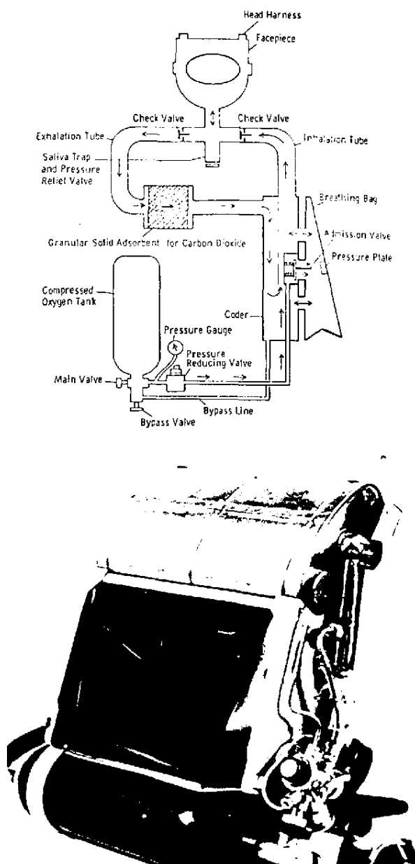
Fig. 5-26. Closed-circuit SCBA.
