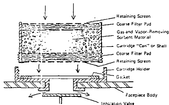
Fig. 5-14. Typical chemical cartridge.
