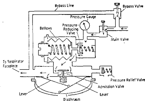
Fig. 5-31. Open-circuit SCBA regulator.
