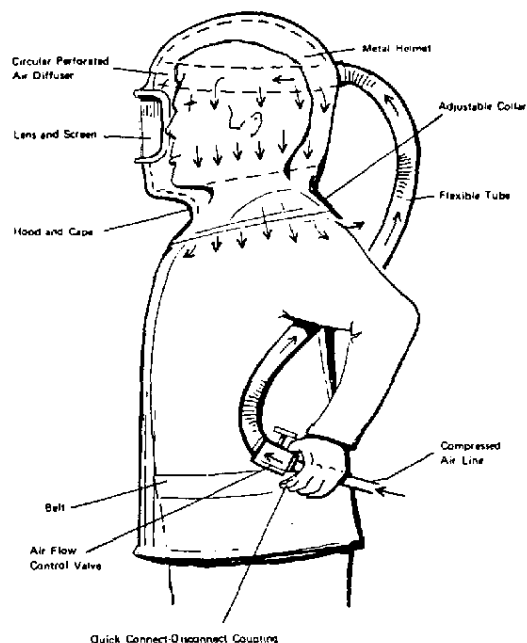
Fig. 5-8. Typical abrasive blasting hood.
