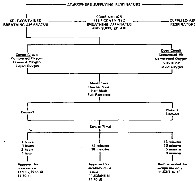
Fig. 5-2(a). Self-contained breathing apparatus.
