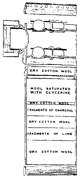
Fig. 2-3. Tyndall and Shaw smoke cap filter.
