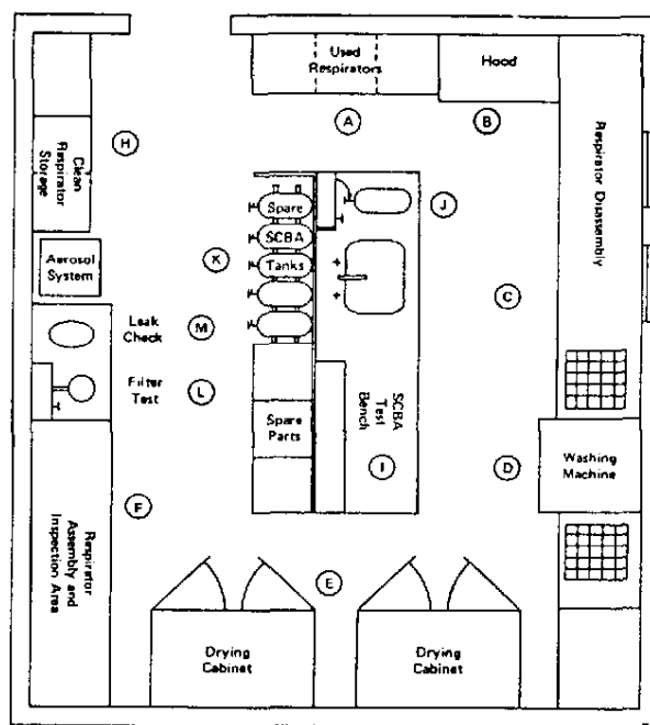
Fig. 9-1. Typical large respirator maintenance facility.
