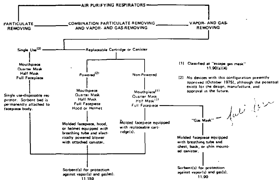
Fig. 5-1(c). Vapor- and gas-removing respirators.
