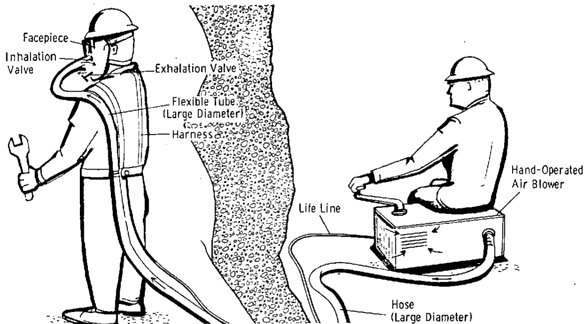
Fig. 5-42. Hose mask respirator with hand-operated blower.
