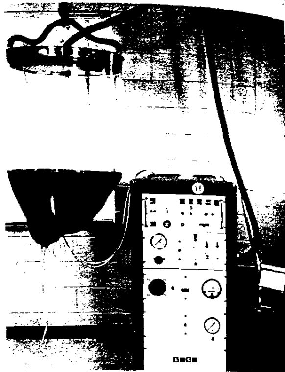
Fig. 8-6. DOP quantitative respirator-fitting test system.
