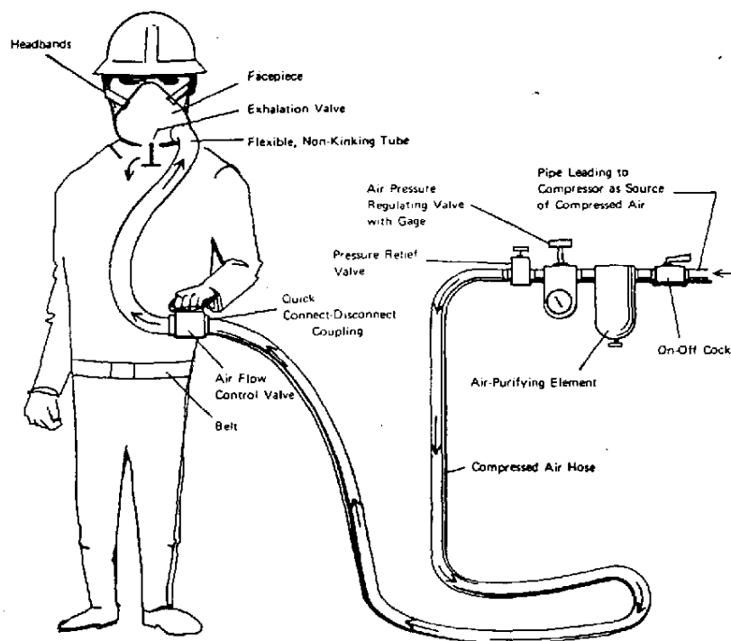
Fig. 5-35. Continuous flow air line respirator.
