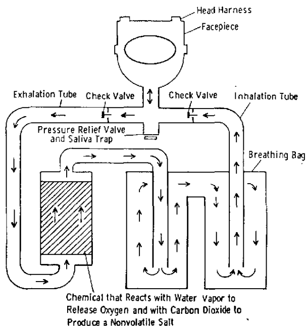
Fig. 5-28. Oxygen-generating closed circuit SCBA.
