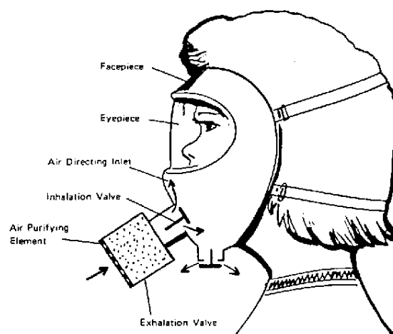
Fig. 5-5. Typical full-facepiece respirator.
