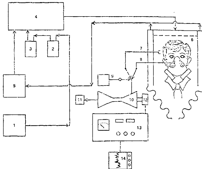
Fig. E-2. DOP quantitative fitting test system schematic.
