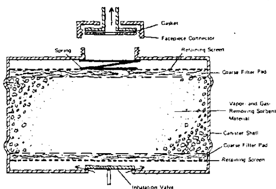
Fig. 5-18. Typical chin-mounted canister.
