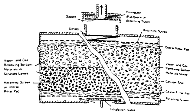
Fig. 5-20. Methods of packing more than one sorbent.
