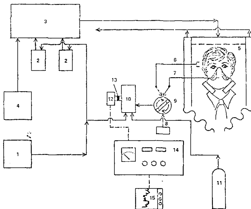
Fig. E-1. NaCl quantitative fitting test system schematic.
