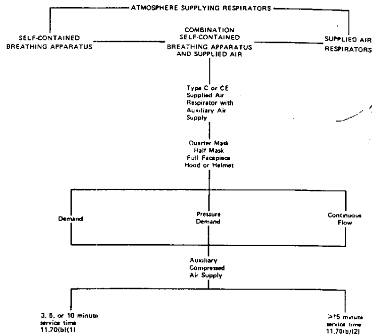
Fig. 5-2(b). Combination SCBA and supplied air respirators.
