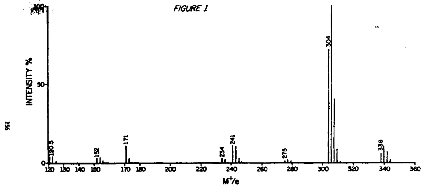
Figure 1 Mass Spectrum resulting from the direct probe analysis, at 30°C and 70 eV, of authenticated 2,3,7,8 tetrachlorodibenzofuran; see Figure 2A for other conditions.
