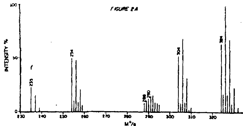
Figure 2A Mass spectrum resulting from GC-MS analysis of 88 \mu l of rat urine. LKB 9000 GC-MS, mass marker 10.3 mass unit. GC column temperature, 209°C; flash heater 235°C; glass coiled column, 6'x1/4" 1.5 OV-17/1.95 QF-1 on 60/80 mesh chromosorb "W" H.P., A.W., DMCS; carrier gas (He) 30 psi and 45 cc/min.; separator, 320°C; source 290°C; energy, 70 eV; accelerating voltage, 3.5 KV; trap current, 60 \mu A; box current, 50 \mu A; leak current, 8 \mu A.
