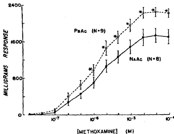
FIG. 1. Concentration-response curve to methoxamine. Helical strips of tail artery from rats treated with sodium acetate (NaAc) or lead acetate (PbAc) were made to contract in response to cumulative addition of methoxamine to muscle bath. Arterial strips from PbAc-treated rats developed more force in response to all concentrations of methoxamine than did those from control rats. Values are means \pm SE; n , no. of rats. *Statistically significant difference between groups at P < 0.05 (unpaired t test).
