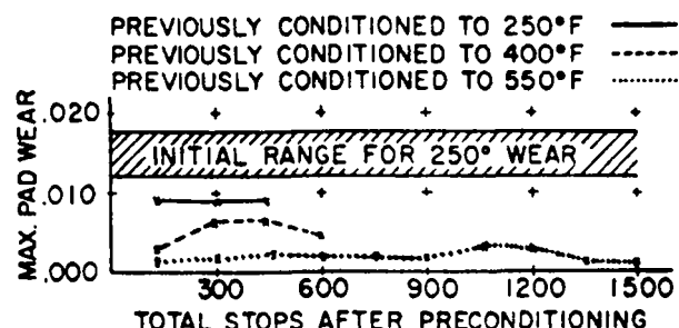
Fig. 5-Effects of preconditioning semi-metallic on subsequent low temperature incremental wear, inertia dynamometer, 1740 lb wheel load, ventilated rotor, all stops from 50 mph, 12 fpsps deceleration
