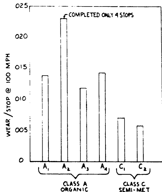
Fig. 4 - Disc pad wear at 100 mph - Full brake dynamometer, Class A versus Class C, 10-stop test
