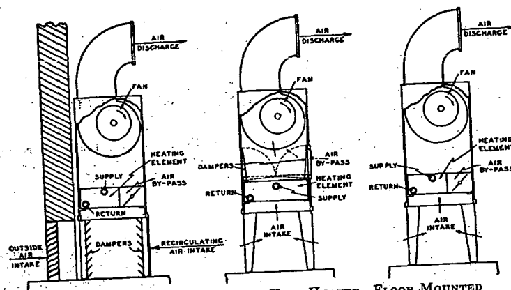
FIG. 1. CENTRIFUGAL FAN TYPE UNIT HEATER—FLOOR MOUNTED
