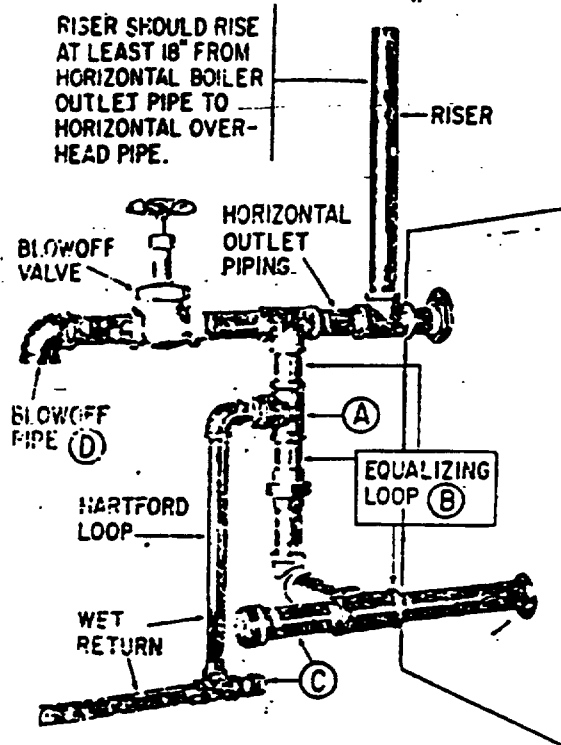
RECOMMENDED PIPING FOR G-23 or G-24 ILLUSTRATED.
