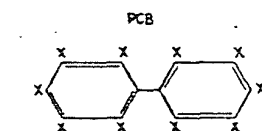
X POSSIBLE POINTS FOR SUBSTITUTION OF CHLORINE (A)
