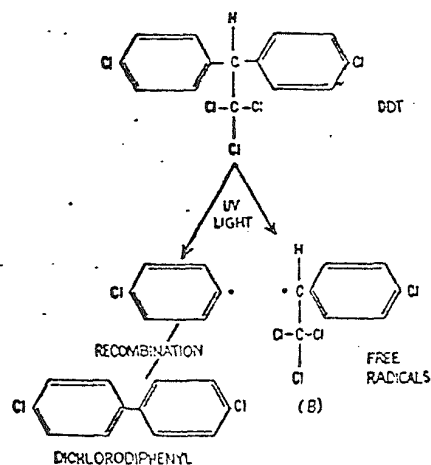
Fig. 1. Basic structure of PCBs (A) and possible reactions of PCBs (B).
