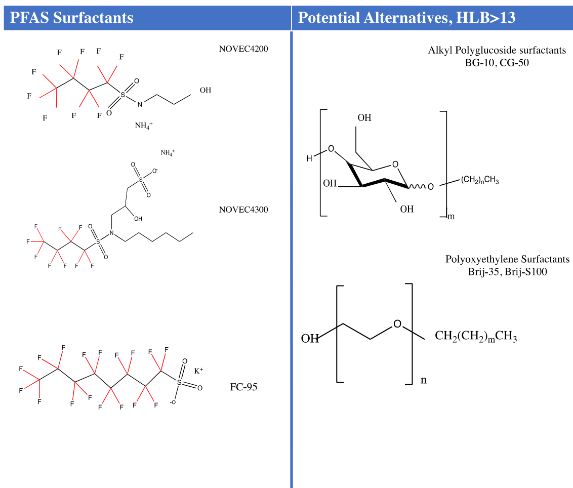
Fig. 5. The molecular structures of the PFAS-based surfactants and the potential alternatives.
