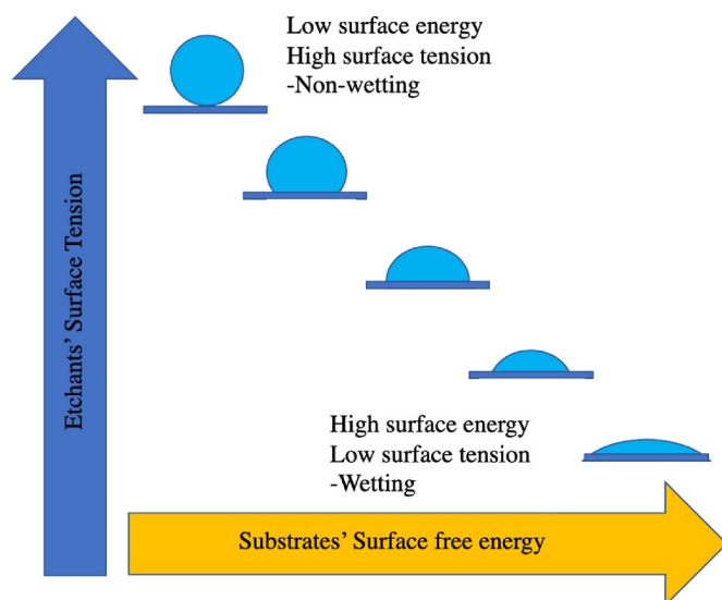
Fig. 6. Relation between Surface tension of the liquid and surface free energy of the substrate in wettability.
