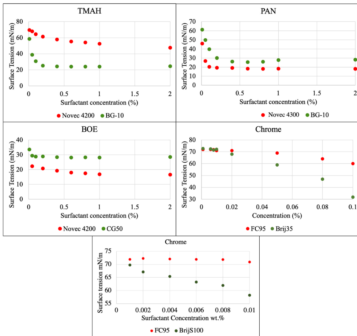
Fig. 3. The surface tension of the etching solution in various PFAS and Alternative surfactant concentrations for (a). TMAH (b). PAN (c). BOE (d) & (e). Chrome etching solutions.
