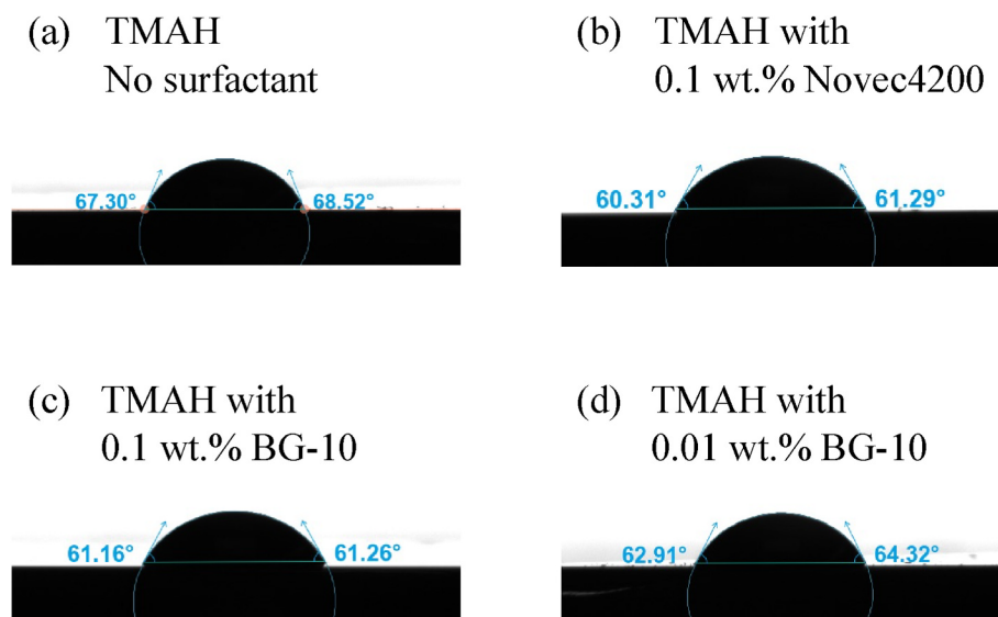
Fig. 4. The contact angle between the photoresist-coated substrate and TMAH etching solution: a. with no surfactant, b. with 0.1 wt% PFAS surfactant Novec 4200 , c. with 0.1 wt% safer alternative BG10 , d. with 0.01 wt% BG10 .
