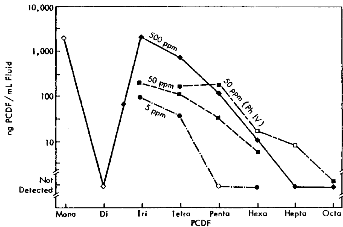
Figure 2. PCDF formation in PCB-spiked mineral oil by homolon (Phase III and Phase IV results). Closed symbols are averages of two values; open symbols are single determinations; missing points are no data. Phase IV data are superimposed on Phase III data, previously published as Figure 22 in Erickson et al. (1984).
