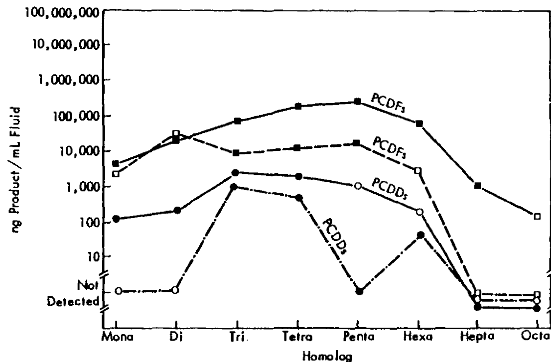
Figure 4. PCDF and PCDD formation from trichlorobenzene transformer fluid (Phase III and Phase IV results). Solid lines are Phase IV results; broken lines are Phase III results, originally published as Figure 25 in Erickson et al. (1984). Closed symbols are averages of two values; open symbols are single determinations.
