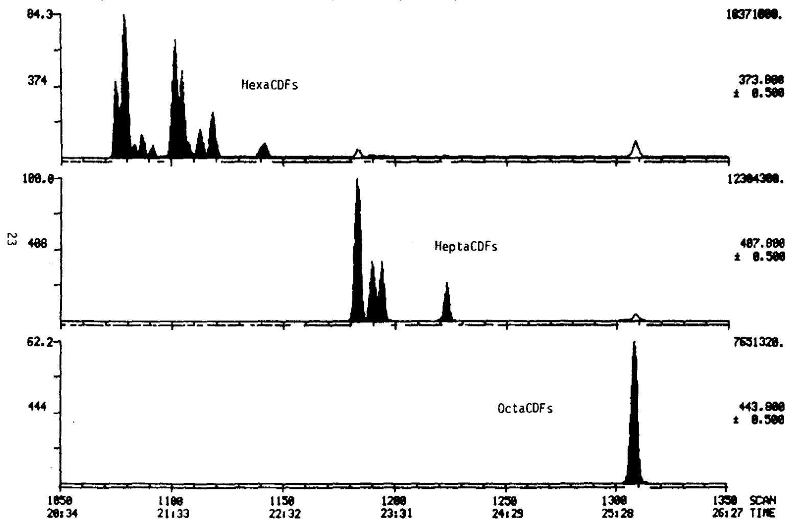
Figure 10. Hexa-, Hepta-, and OctaCDFs in sample 11-39-100-OCDF.
