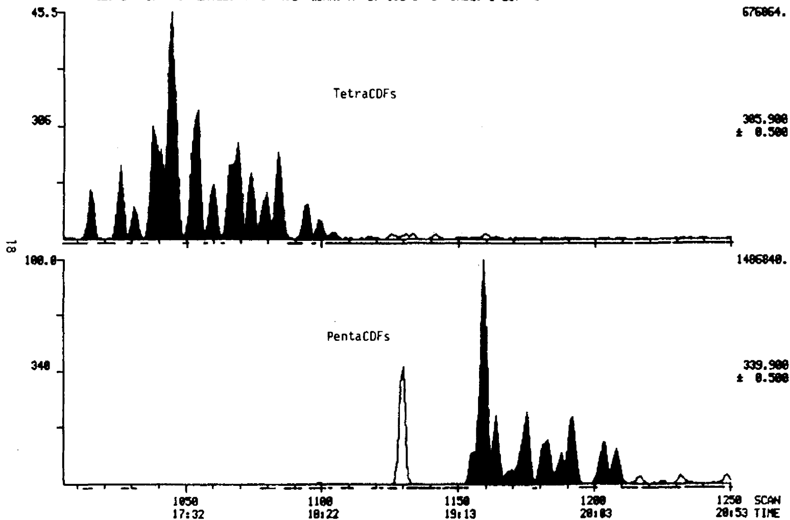
Figure 6. Tetra- and PentaCDFs in sample 11-19-94-WEC.
