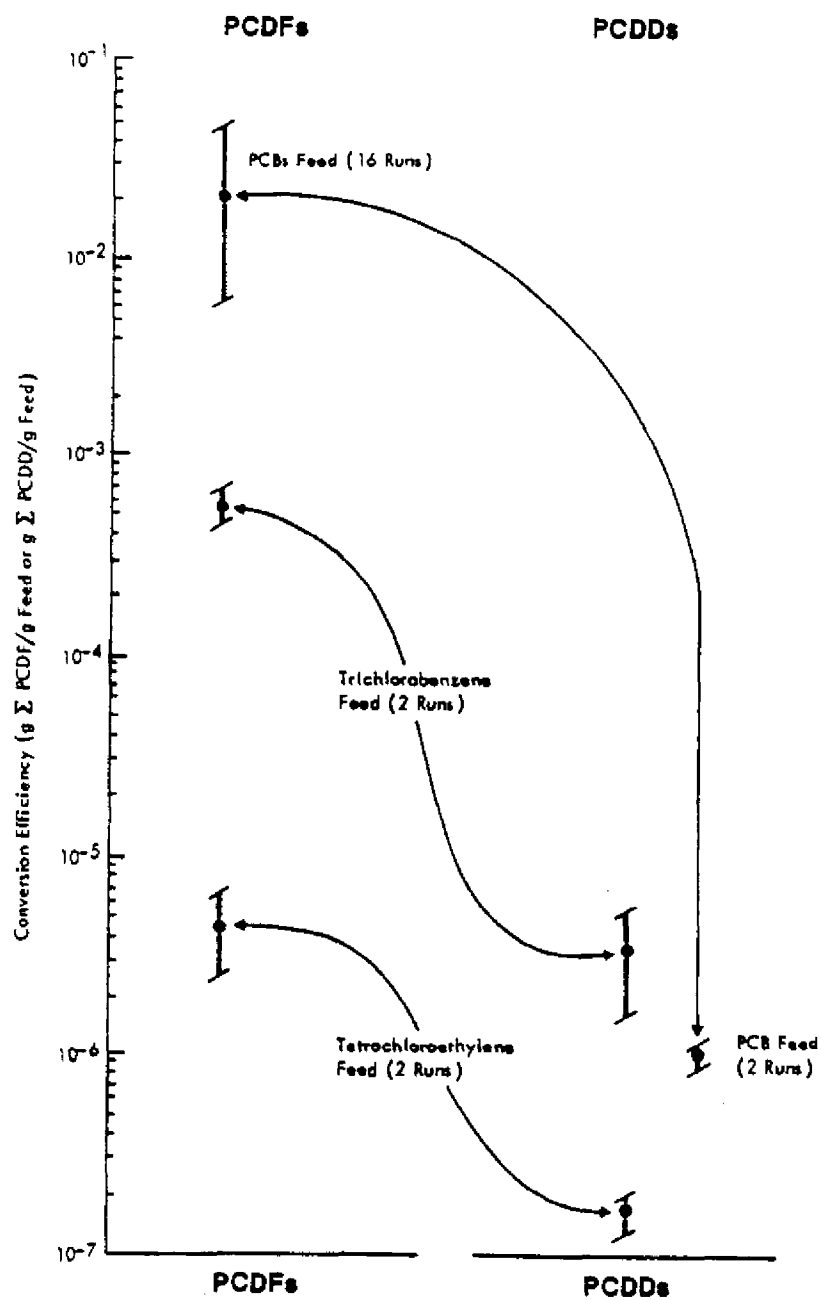
Figure 1. Summary of conversion efficiencies for total PCOFs from Phase III and Phase IV runs.
