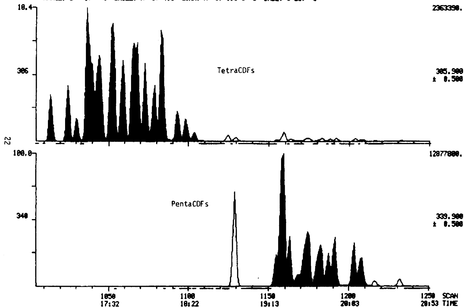
Figure 9. Tetra- and PentaCDFs in sample 11-30-100-OCDF.
