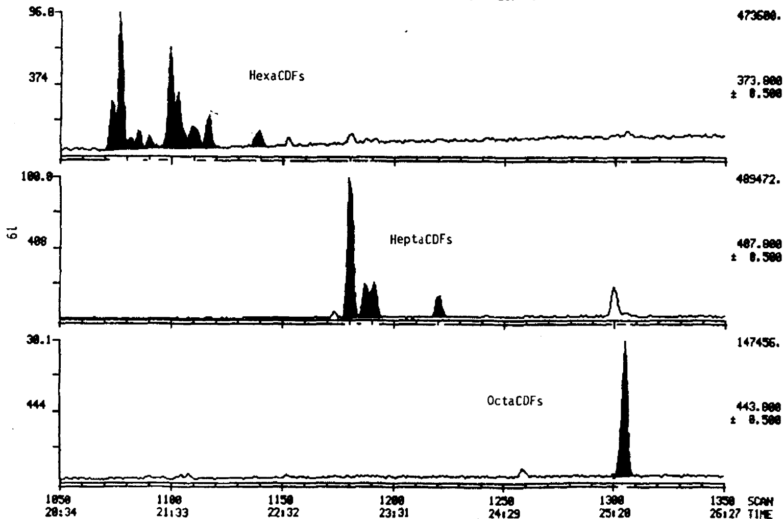
Figure 7. Hexa-, Hepta-, and OctaCDFs in sample 11-19-94-WEC.
