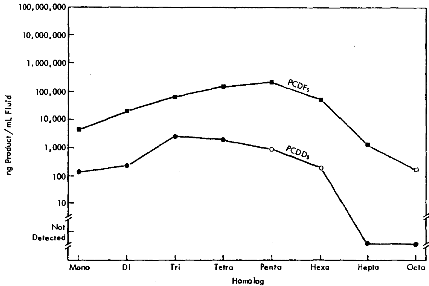
Figure 3. PCDF and PCDD formation from trichlorobenzene transformer fluid (Phase IV results). Closed symbols are averages of two values; open symbols are single determinations.
