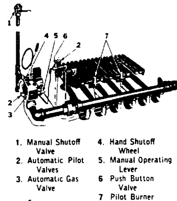
FIG. 25—Control Arrangement
