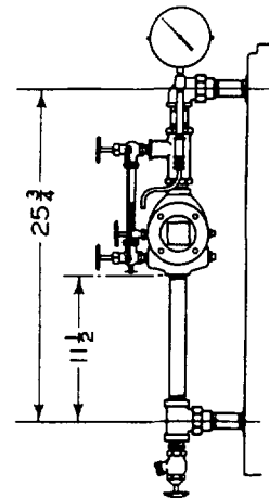
FIG. 10—Low Water Cutoff
