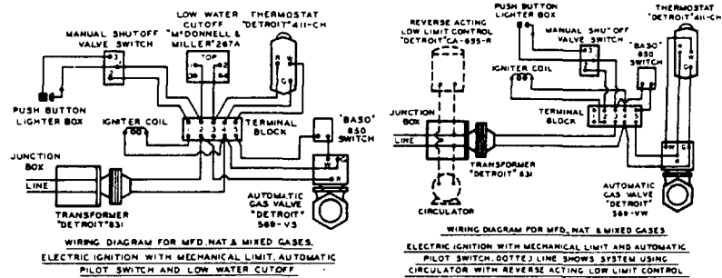
FIG. 13—Wiring Diagrams (Electric Ignition)
