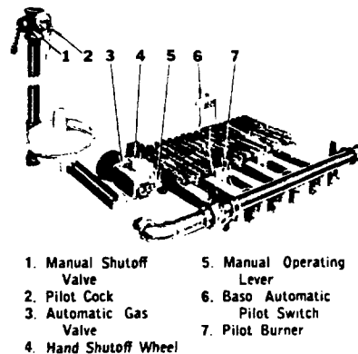
FIG. 24—Control Arrangement
