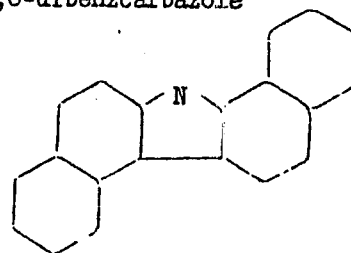
1,2,5,6-dibenzcarbazole
