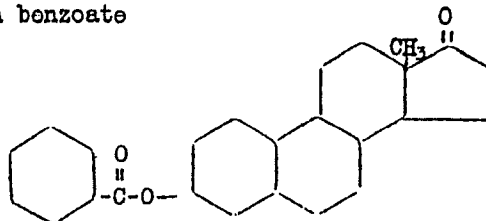
Equilenin benzoate
