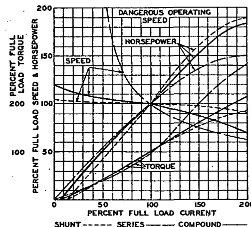
FIG. 1. CHARACTERISTICS OF DIRECT CURRENT MOTORS
