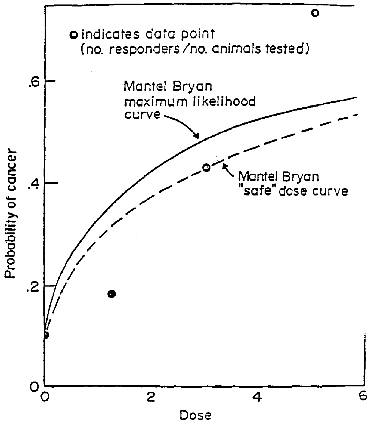
Figure 2. Typical fit of Mantel-Bryan curve to experimental data (from Crump, 1977b).
