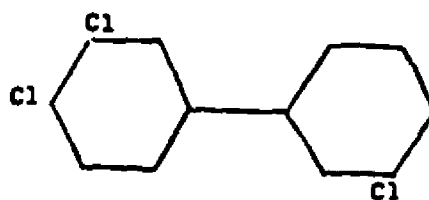
3,3',4-trichlorobiphenyl
