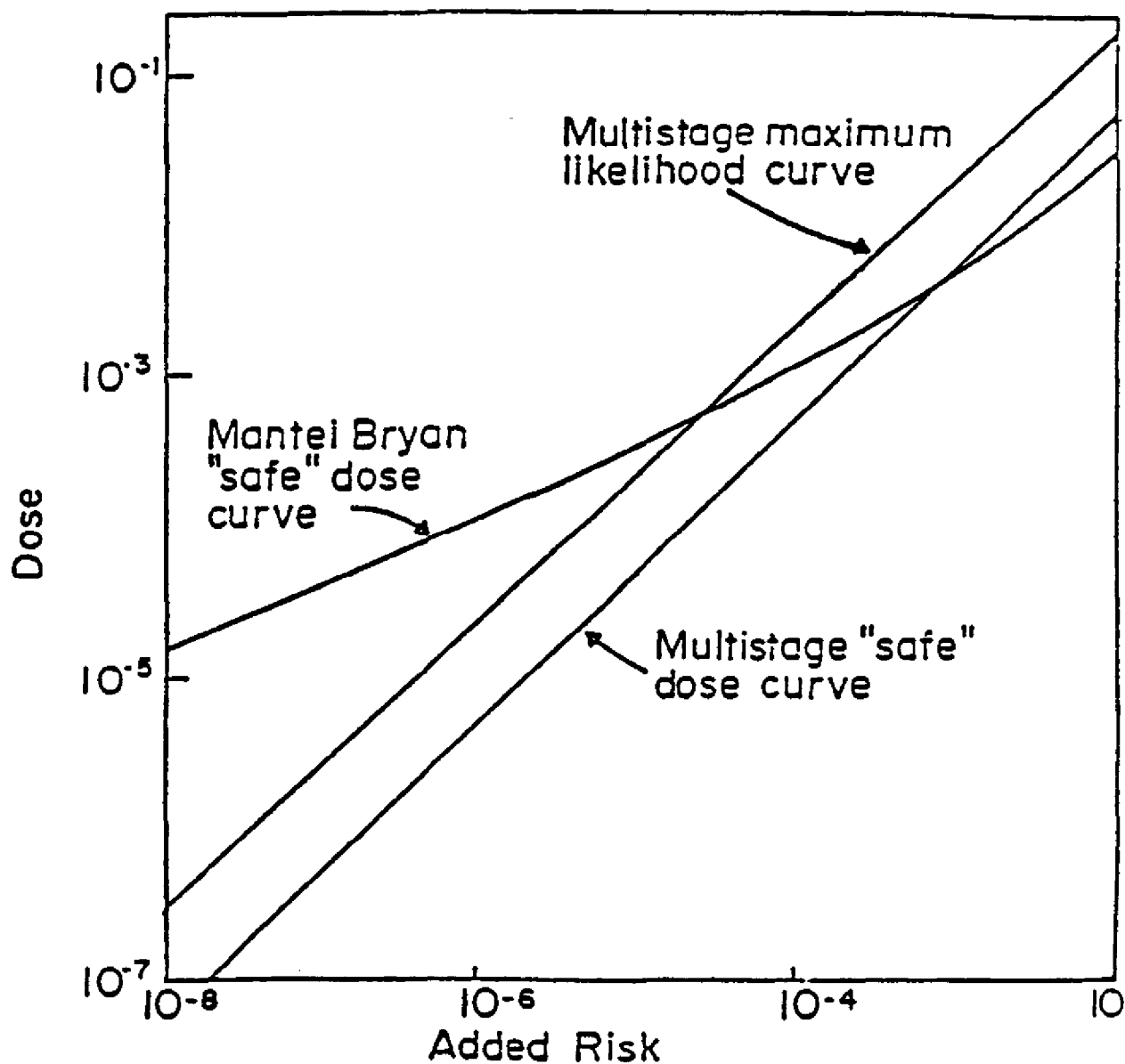
Figure 4. Comparisons of 'safe' doses computed from the Mantel-Bryan procedure and from a procedure based upon the multistage model (from Crump, 1977b).
