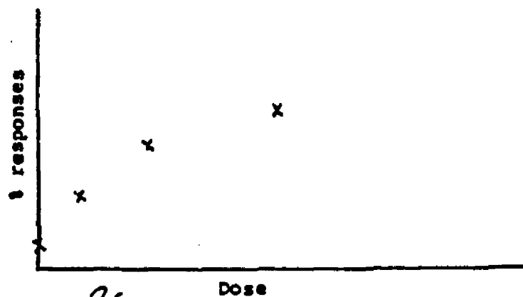
36 Figure 3b. Example of Data Exhibiting Downward Curvature
