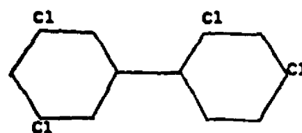
2',3,4',5-tetrachlorobiphenyl
