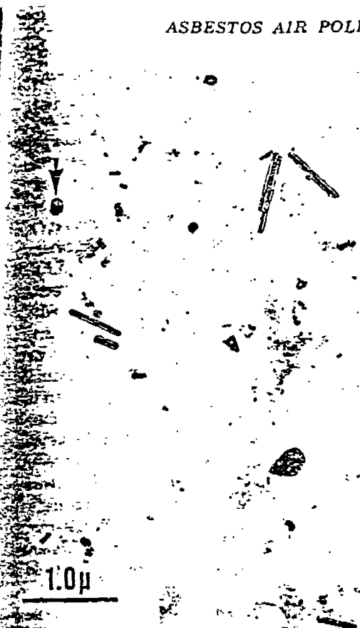
Fig 4.—Single, short fibrils collected 3/16 of mile downwind of chrysotile source. Arrow indicates position of clay particle.
