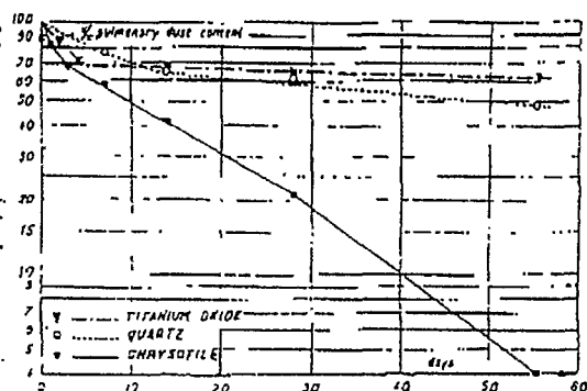
FIGURE 5. Plot of pulmonary dust content: ( \Delta ) titanium oxide; (o) quartz; (*) chrysotile.
