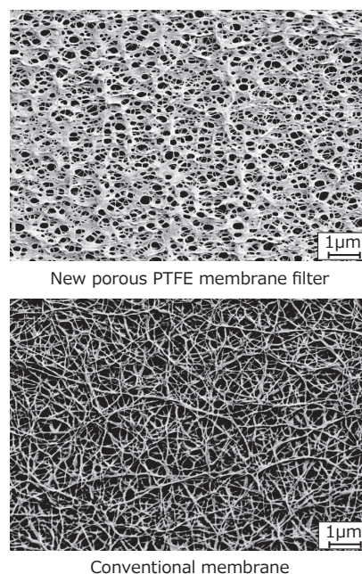
Fig. 6. SEM images of the new porous PTFE membrane and a conventional membrane (surfaces)
