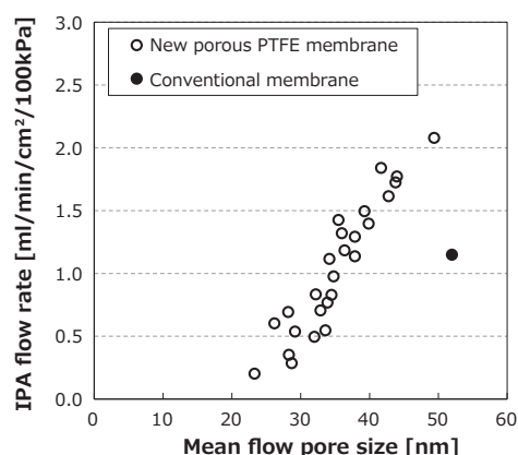
Fig. 5. Mean flow pore size and IPA flow rate of the new PTFE porous membrane and a conventional membrane
