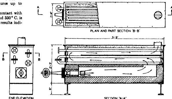
Figure 1. Heater
