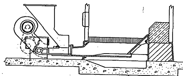
FIG. 4. UNDERFEED SIDE CLEANING STOKER
