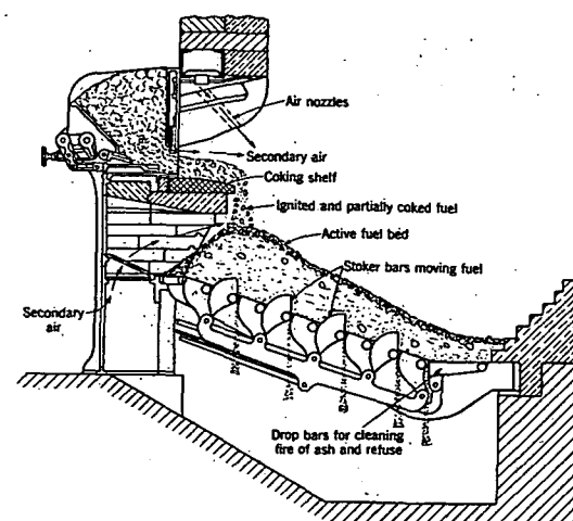
FIG. 3. OVERFEED INCLINED GRATE STOKER
