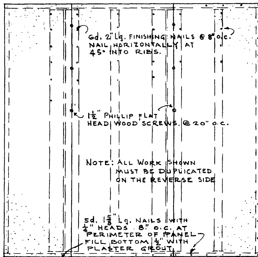
ELEVATION OF PANEL
