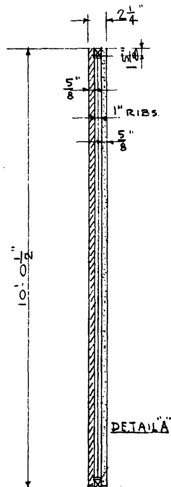
SECTION
