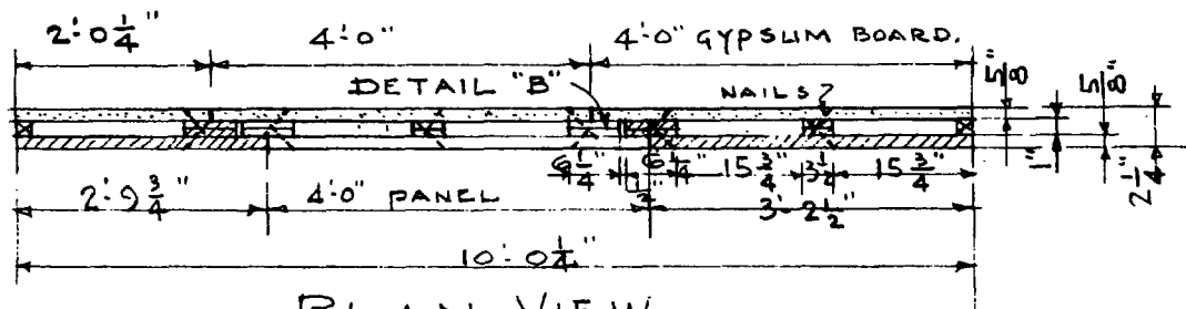
PLAN VIEW Scale 1/2" = 1'-0"
