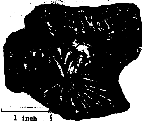
D. GRAPHITE ROSETTE Crystal Graphite Mine
