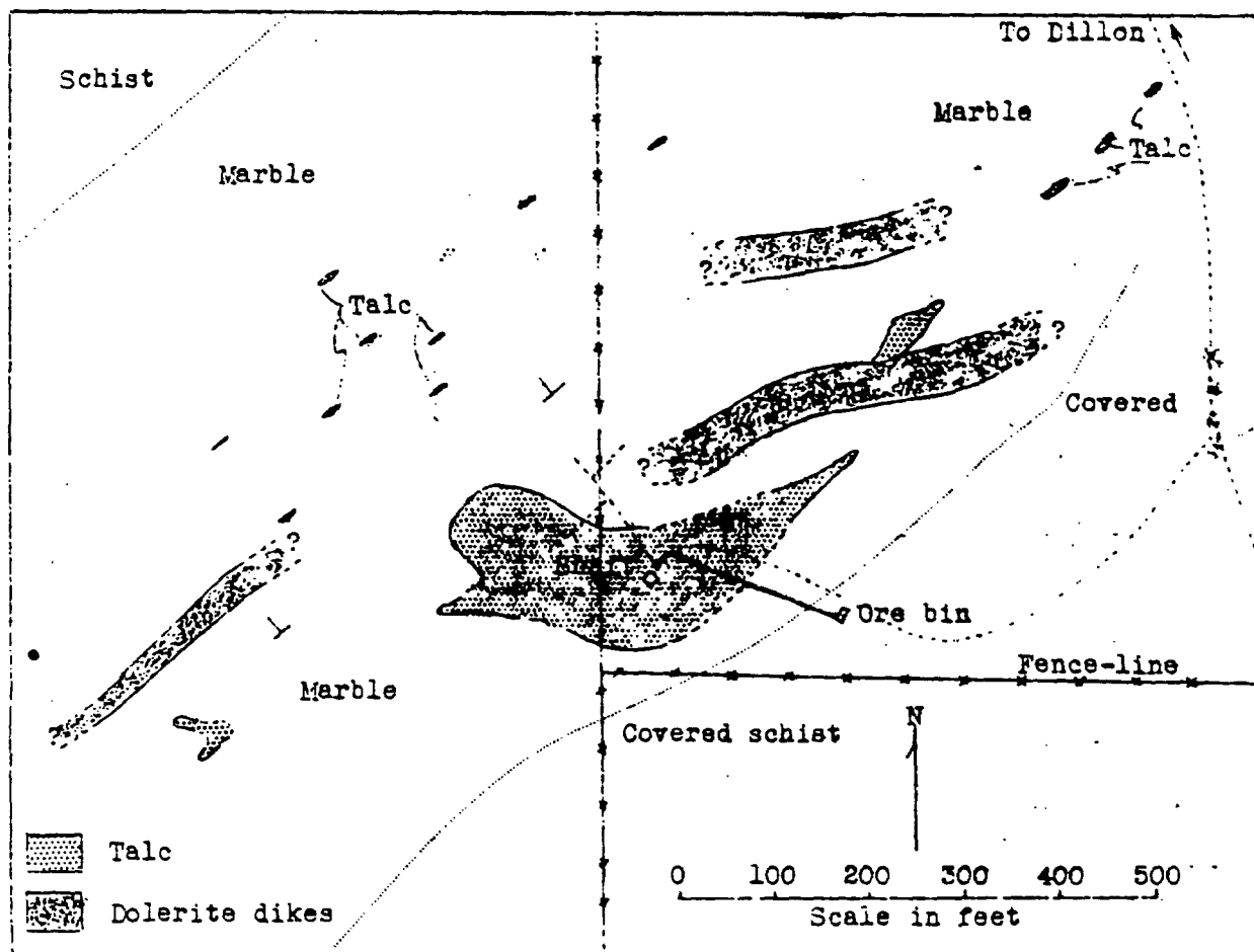
Figure 1.--Map of Keystone talc deposit on Carter Creek, Beaverhead County.
