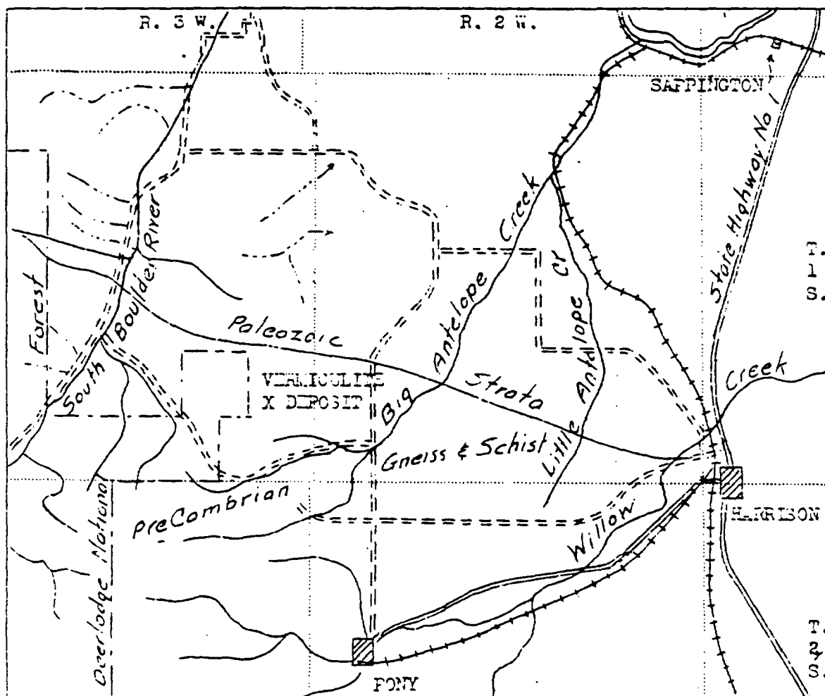
Figure 7.--Map showing location of vermiculite deposits near Pony.
