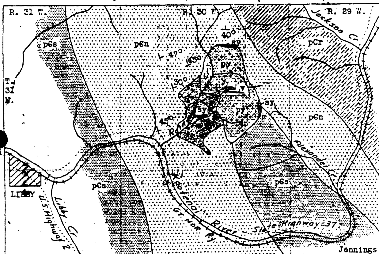
Figure 4.—Geologic map of Libby vermiculite deposit, Lincoln County. pCs, Spokane formation; pCn, Newland formation; pCr, Ravalli formation, sy, syenite; py, pyroxenite; v, biotite rock altered to vermiculite.
