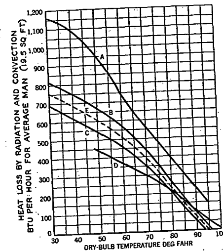
FIG. 6. RELATION BETWEEN RADIATION AND CONVECTION LOSS FROM THE HUMAN BODY AND DRY-BULB TEMPERATURE FOR STILL AIR. 14
