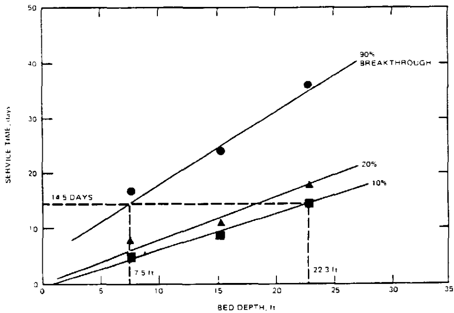
Figure D.2 SERVICE TIME AS A FUNCTION OF BED DEPTH
