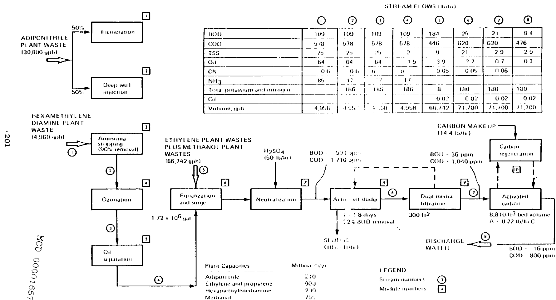
TREATMENT OF MULTIPLANT WASTES
