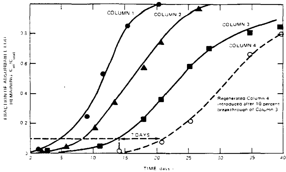
Figure D.1 BREAKTHROUGH CURVES FOR THREE COLUMNS IN SERIES
