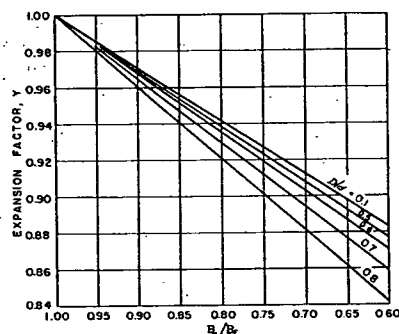
FIG. 5. EXPANSION FACTOR FOR AIR AND OTHER DIATOMIC GASES APPLICABLE TO FLANGE, RADIUS AND VENA CONTRACTA TAPS
