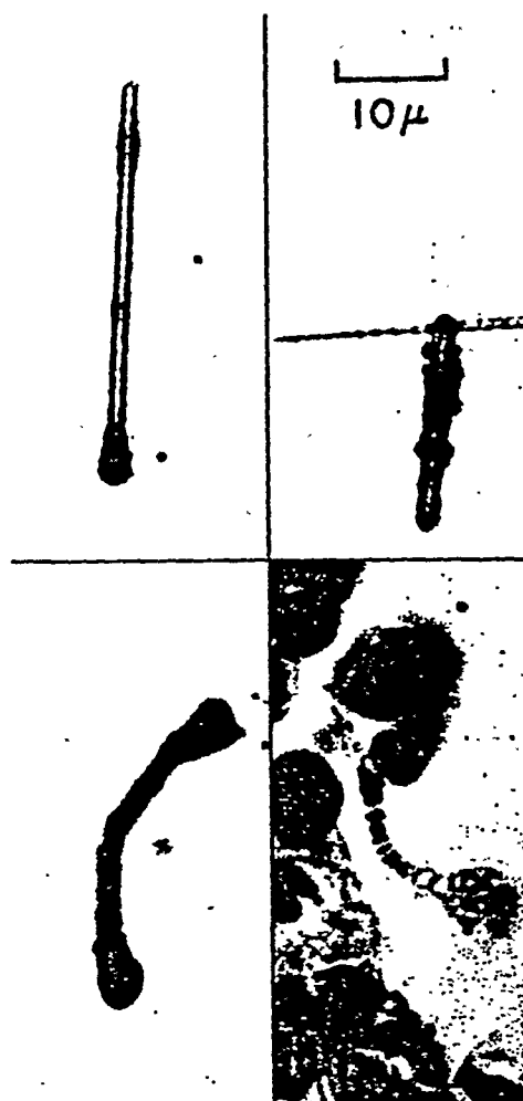
Fig 4.—Ferruginous bodies formed in response to other filamentous dusts and stained for iron (Perls' test). The central fiber (top, left and right) is silicon carbide; and (bottom left) tremolite (tafc) ( \times 1,110 ).
