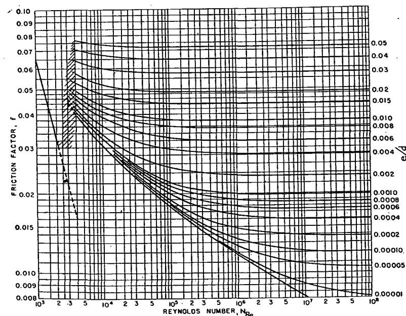
FIG. 4. RELATION BETWEEN FRICTION FACTOR AND REYNOLDS NUMBER
