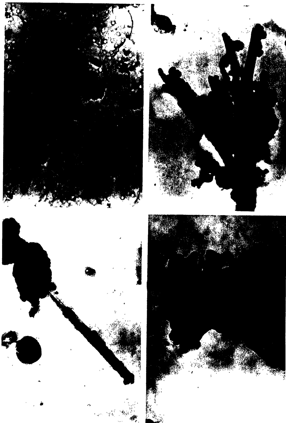
Fig. 1. Asbestos fibers in brake drum dust. Scanning transmission electron microscopy at different magnifications: Upper left, \times 6,300 ; upper right, \times 35,000 ; lower left, \times 50,000 ; lower right, \times 60,000 . Whereas at a magnification of \times 6,300 (lower borderline = 14 \mu\text{m} ) only a few fibers are visible, at higher magnifications numerous unit fibrils are observed.
