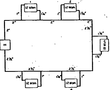
FIG. 7. A ONE-PIPE GRAVITY CIRCULATION SYSTEM
