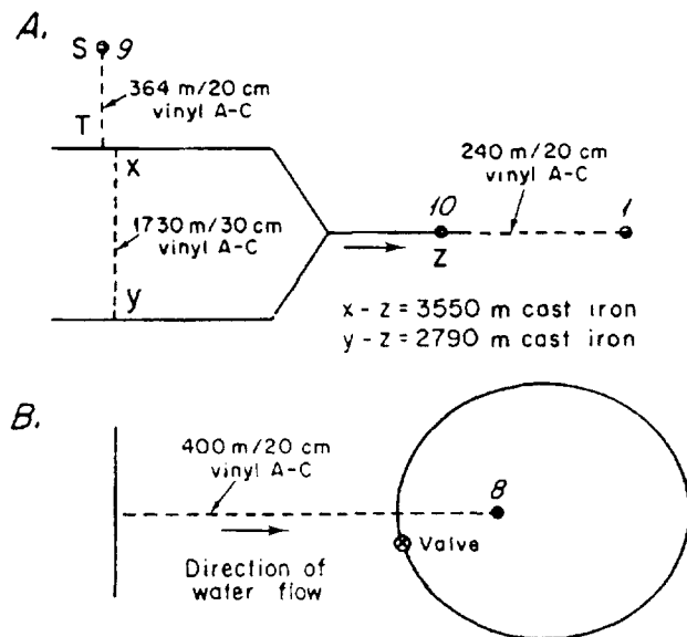
FIGURE 1. Schematic diagram (not to scale) showing pipe networks leading to sampling locations 1, 9, and 10 (A) and location 8 (B). ---- Vinyl-coated A-C; — cast iron.
