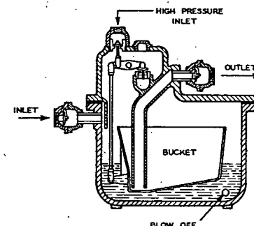
FIG. 32. LIFTING TRAP
