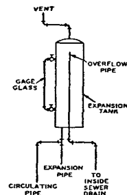
Fig. 14... An Open Expansion Tank
