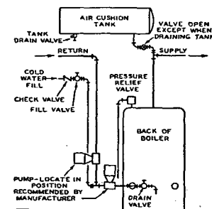
Fig. 15... A Closed Expansion Tank
