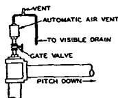
Fig. 12... Typical Automatic Air Vent Valve Installation
