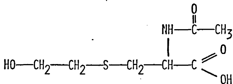
(A) N -ACETYL( S -2-HYDROXYETHYL)CYSTEINE
