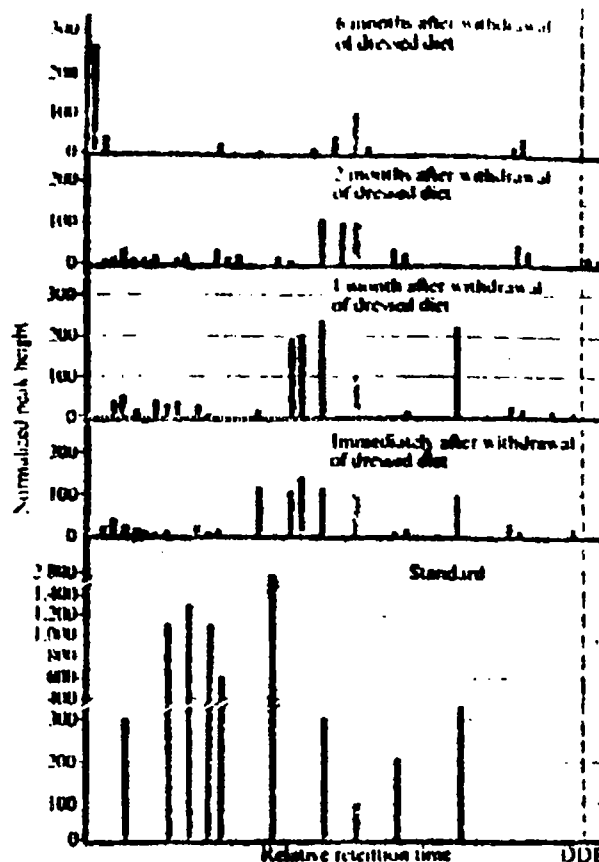
Fig. 2 Gas-liquid chromatographic "spectra", normalized to a common peak (stippled column) of 'Aroclor 1242' standard and mean pigeon liver residues following feeding at 500 p.p.m. in diet for 20 days.
