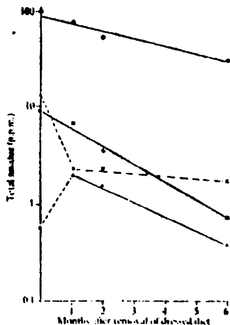
Fig. 1 Mean total levels of PCB in pigeon tissues following feeding of 'Aroclor 1242' at 500 p.p.m. in diet for 20 days.
