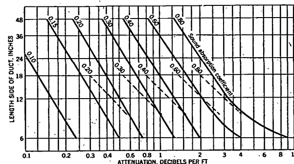
FIG. 3. SOUND ATTENUATION FOR VARIOUS ABSORBING DUCT LINERS
