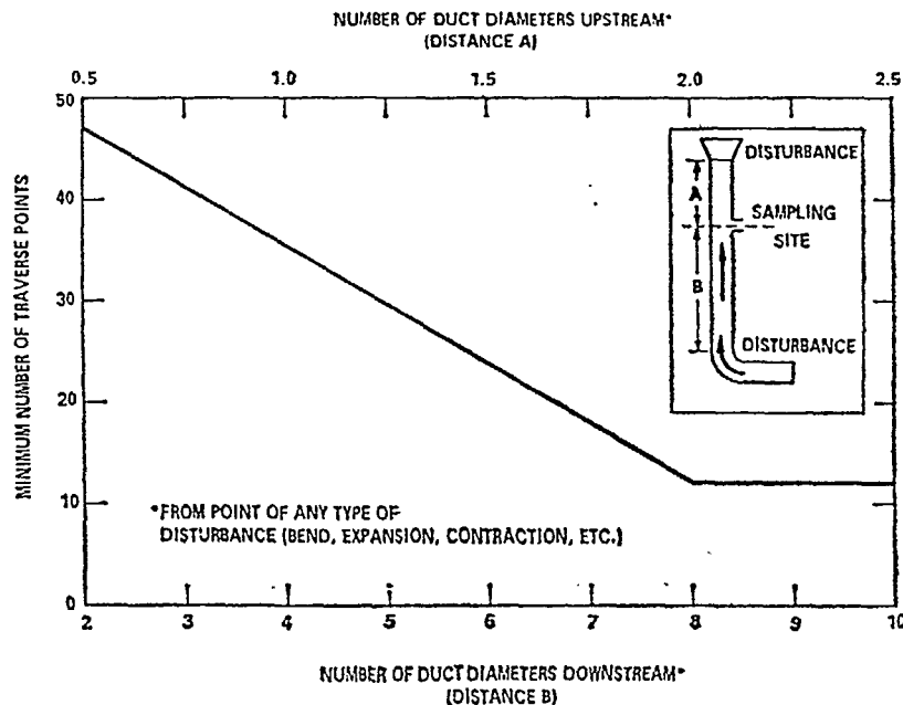
Figure 102-3. Minimum number of traverse points.
