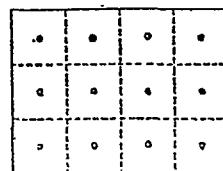
Figure 101-5. Cross section of rectangular stack divided into 12 equal areas, with traverse points at center of each area.
