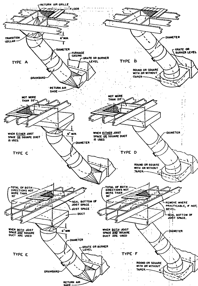
FIG. 5. TYPICAL ARRANGEMENTS OF RETURN-AIR DUCT SYSTEMS
