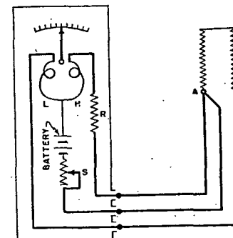
FIG. 2. TYPICAL RESISTANCE THERMOMETER CIRCUIT AND CONNECTIONS
