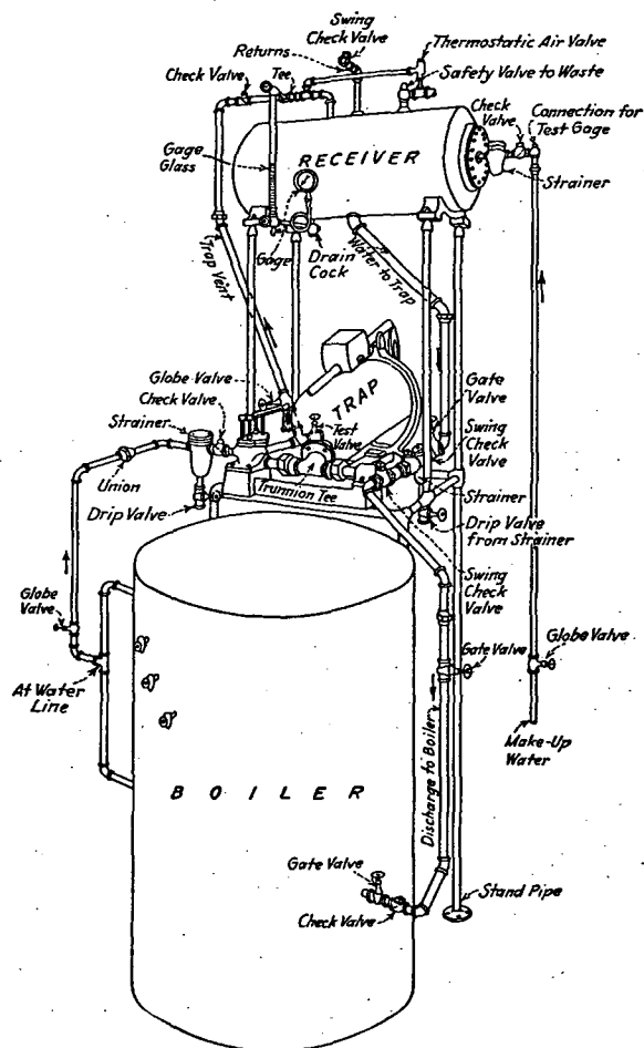
FIG. 8. RETURN TRAP AND RECEIVER FOR AUTOMATIC BOILER FEED
