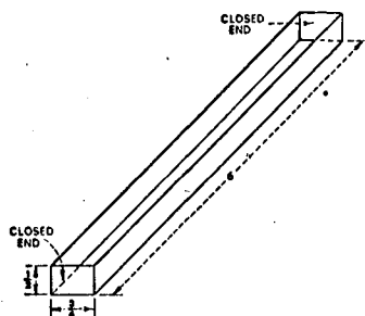
FIG. 1—Assembly for Testing Flow in Class A Compounds.
