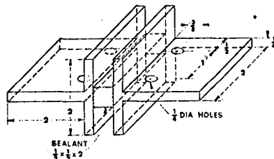
FIG. 4—Assembly for Testing Adhesive Strength to T-Sections.
