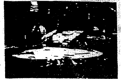
Molten metal is pumped to the desilverizing kettle where zinc is added
