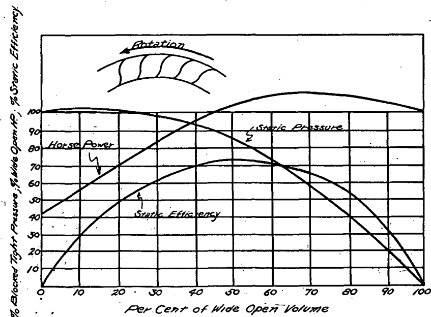
FIG. 5. OPERATING CHARACTERISTICS OF A FAN WITH A DOUBLE CURVED BLADE.
