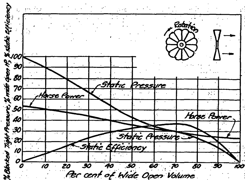
FIG. 2. OPERATING CHARACTERISTICS OF A DISC OR PROPELLER FAN.
