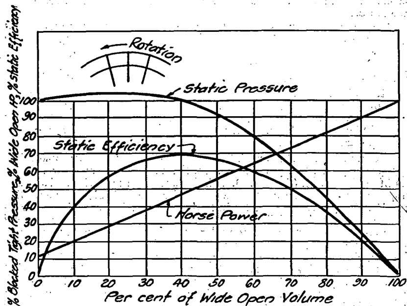
FIG. 3. OPERATING CHARACTERISTICS OF A FAN WITH STRAIGHT BLADES.
