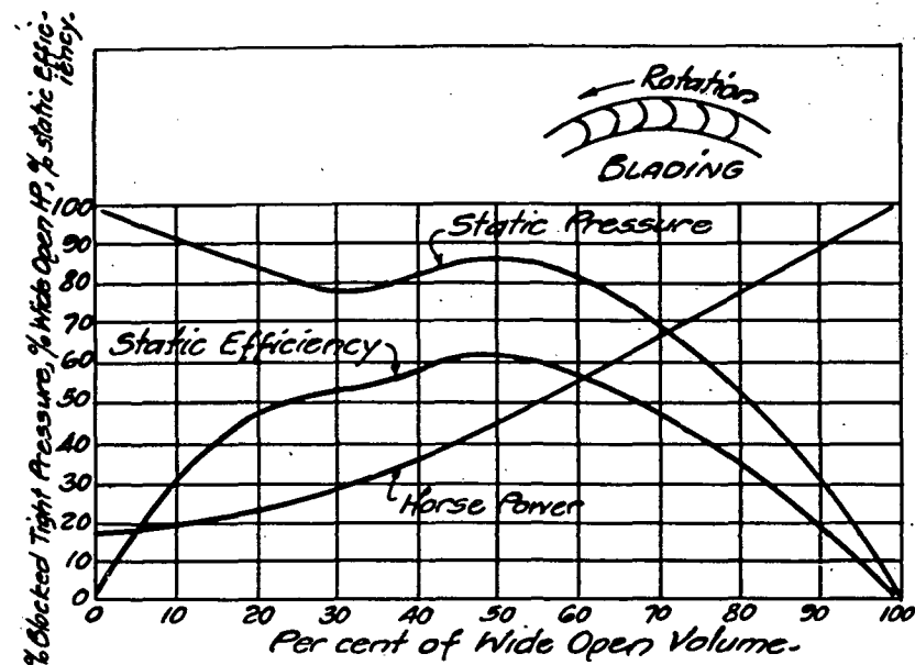
FIG. 4. OPERATING CHARACTERISTICS OF A FAN WITH BLADES CURVED FORWARD.
