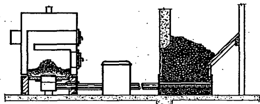
FIG. 2. UNDERFEED STOKER, BIN FEED TYPE, CLASS 1
