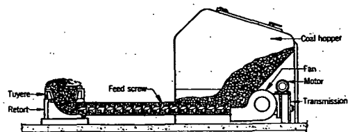
FIG. 1. UNDERFEED STOKER, HOPPER TYPE, CLASS 1
