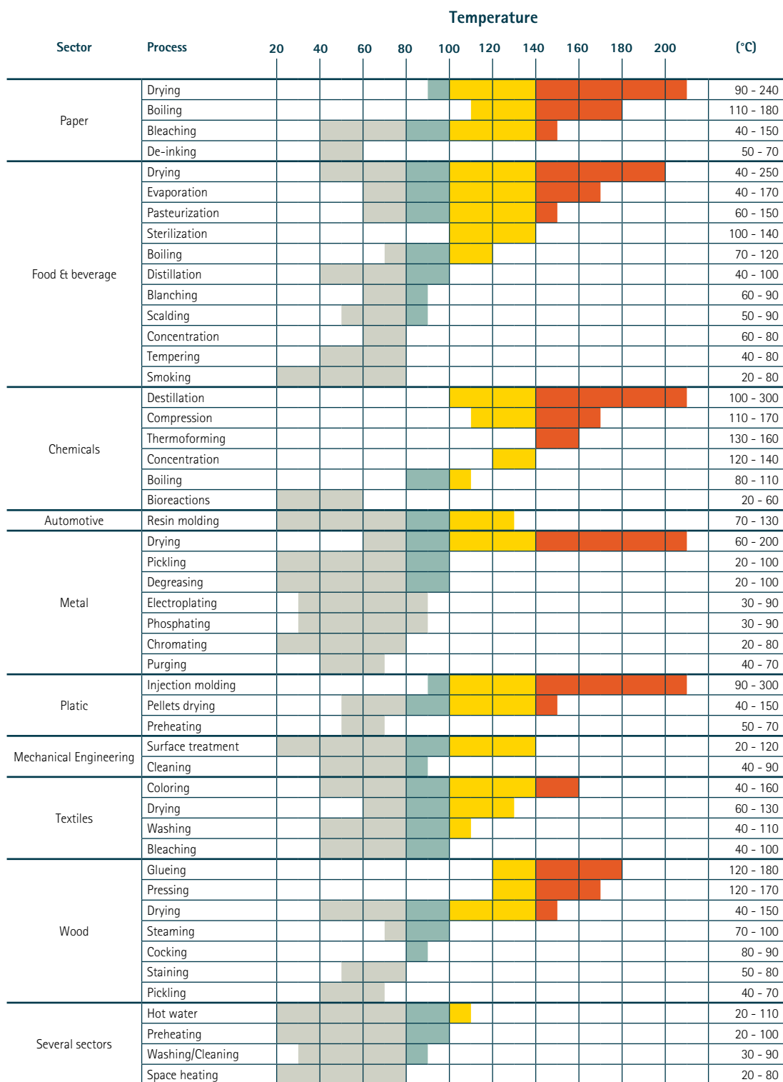
Figure 25 TEMPERATURE RANGES OF DIFFERENT INDUSTRIAL PROCESSES
