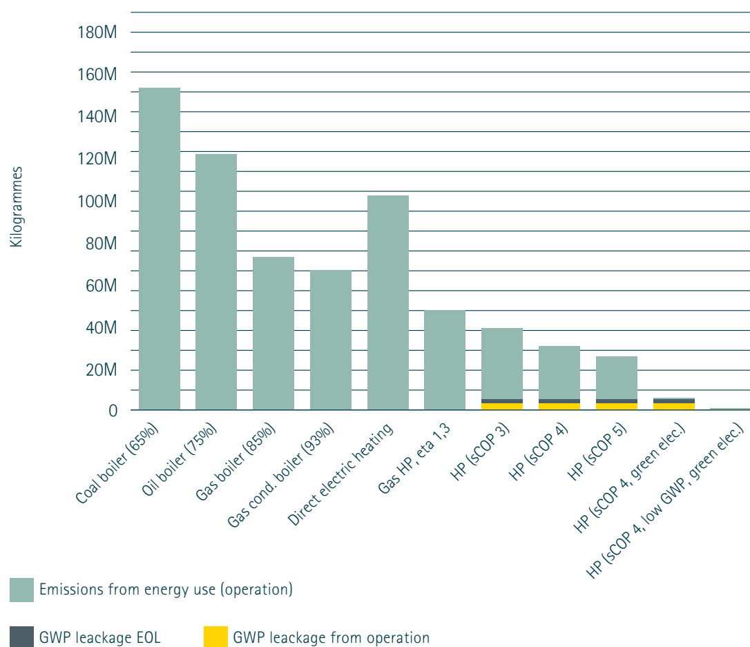
Figure 21 EXAMPLES OF TOTAL ENVIRONMENTAL WARMING IMPACT (LIFETIME)
