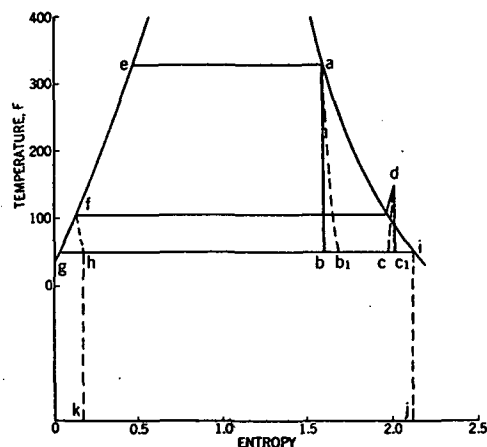
FIG. 5. STEAM EJECTOR TEMPERATURE-ENTROPY DIAGRAM
