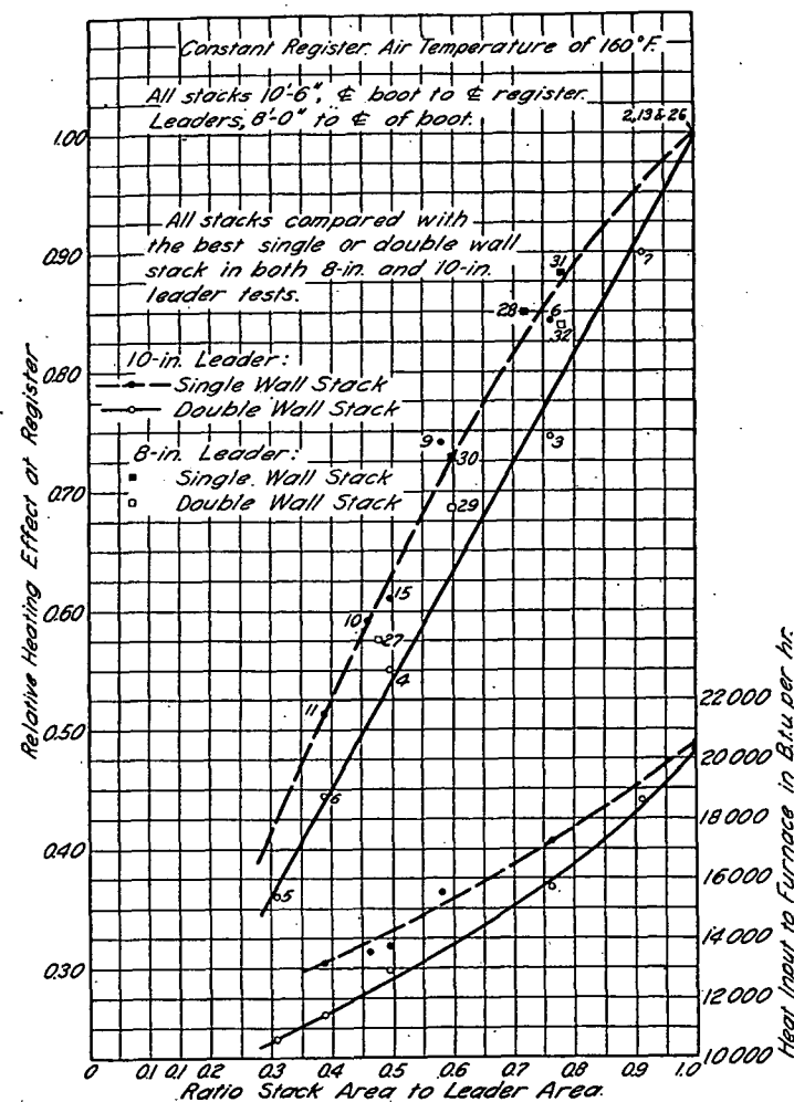
FIG. 3. RELATIVE HEATING EFFECT OF STACKS AT CONSTANT REGISTER AIR TEMPERATURE
