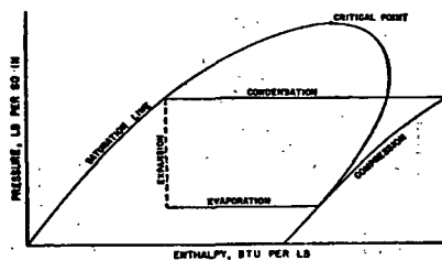
FIG. 3. PRESSURE-ENTHALPY DIAGRAM FOR SIMPLE SATURATION CYCLE
