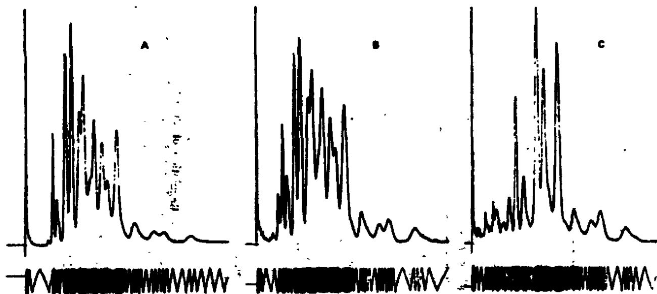
Fig. 1. Typical g/c chromatograms: A = commercial grade Aerosil 1204 standard, B = Aerosil 1204 extracted from sludge, and C = the Aerosil 1204 residue extracted from the milk of cows. These chromatograms were from an F & M model 408 with a ^{63}\text{Ni} detector, A 2.44-m glass column of 4% DC-200 and 6% QF-1 (1:1) on Gas Chrom Q (80/100 mesh) with argon-methane (95:5) as carrier and purge. Operating conditions were: flash heater 230^\circ\text{C} , column oven 210^\circ\text{C} , detector 300^\circ\text{C} , and gas flow 40 to 50 ml/min (WILLETT 1973 c).
