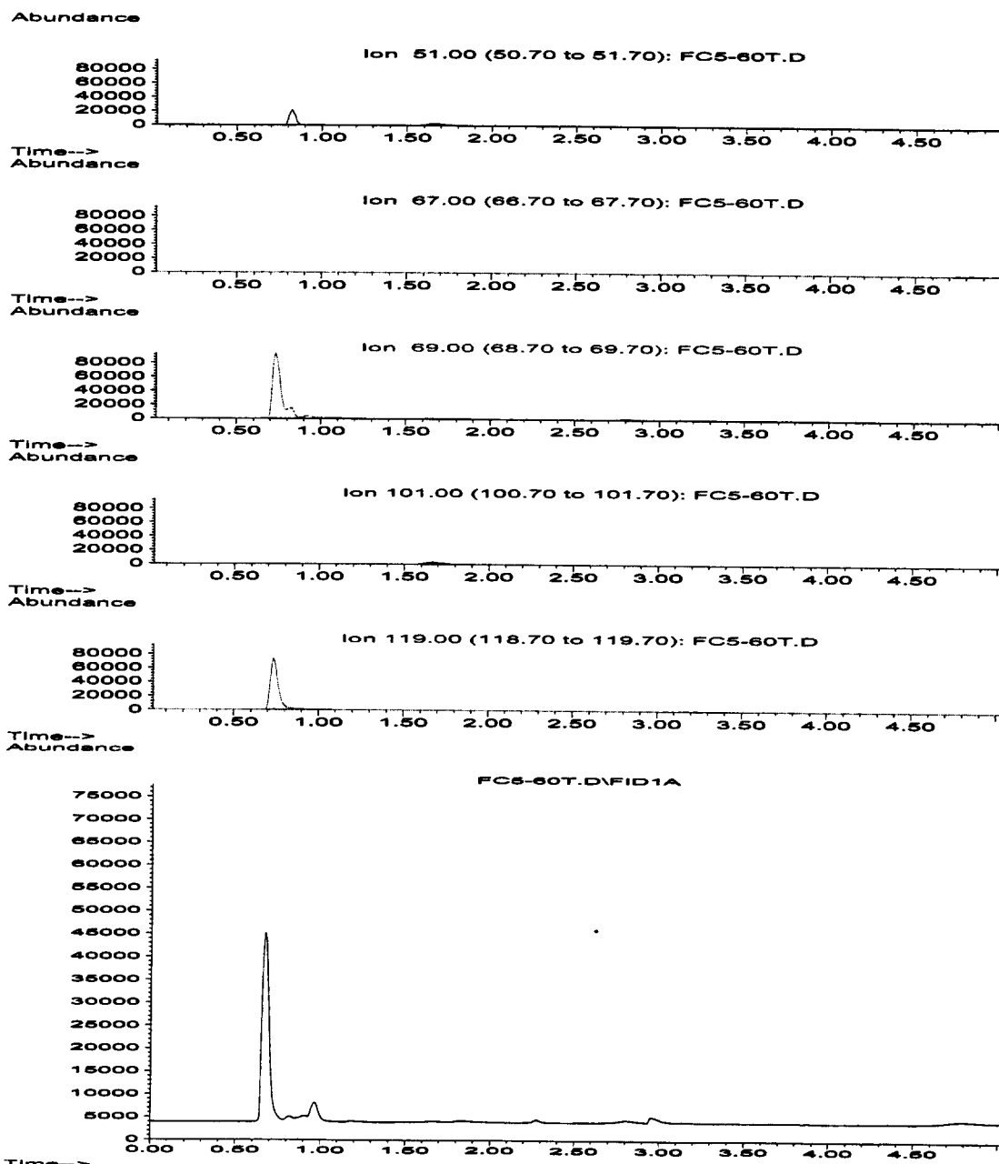
Figure 5.8.2. Extracted Ions ( \text{CF}_2\text{H-51} , \text{SOF-67} , \text{CF}_3\text{-69} , \text{CF}_2\text{CF}_2\text{H-101} , and \text{C}_2\text{F}_5\text{-119} ) and Corresponding HFID Signal for Combustion of PFXS at 600°C (off-line sample)
