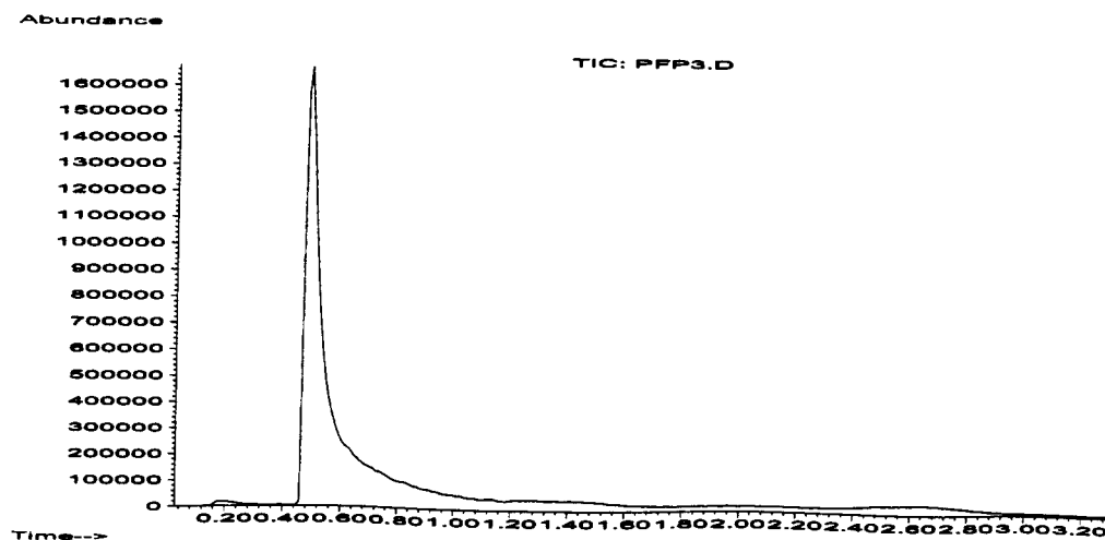
Figure 36. Total Ion Chromatogram for HFP (7,000 ppm)
