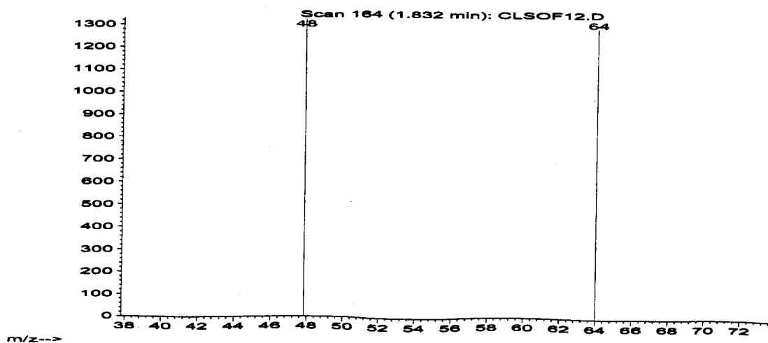
Figure 15. Mass Spectra for \text{SO}_2 (78.5 ppm)
