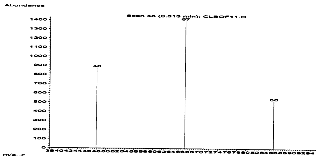
Figure 17. Mass Spectra for \text{SOF}_2 (30.3 ppm)
