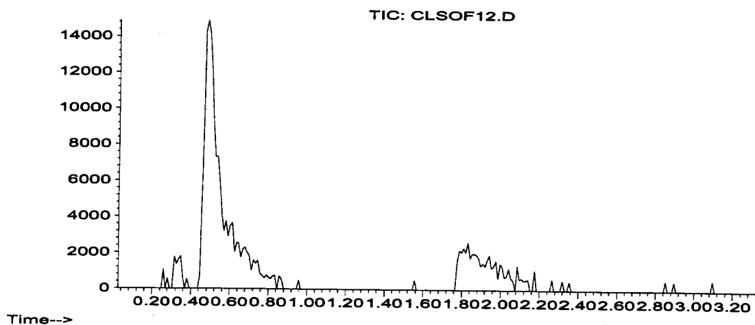
Figure 14. Total Ion Chromatogram for \text{SOF}_2 (151.7 ppm) and \text{SO}_2 (78.5 ppm)
