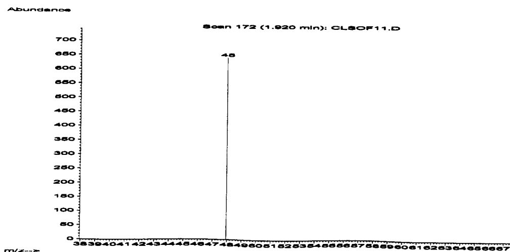
Figure 18. Mass Spectra for \text{SO}_2 (15.7 ppm)
