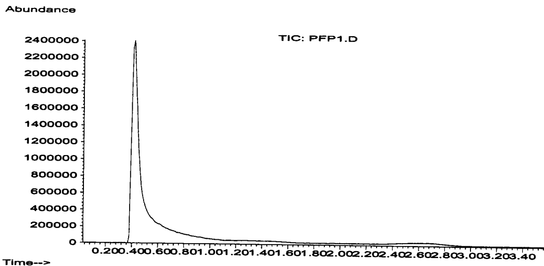
Figure 34. Total Ion Chromatogram for Hexafluoropropene (HFP) (10,000 ppm)
