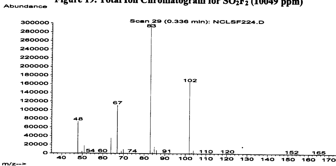
Figure 20. Mass Spectra for SO 2 F 2 (10049 ppm)
