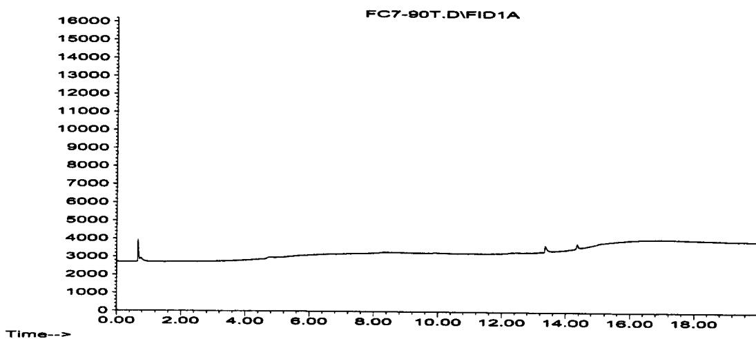
Figure 5.8.4. HFID Signal for PFOS at 900°C (off-line sample)
