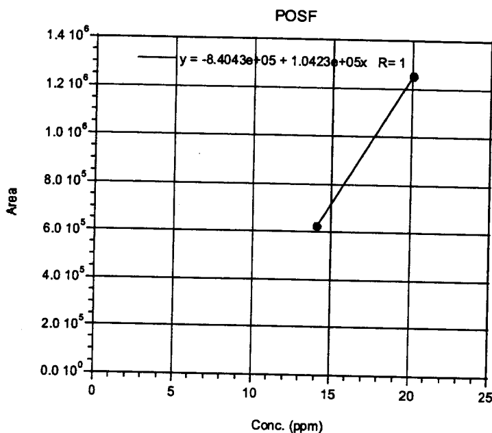
Figure 5. Calibration Plot for POSF
