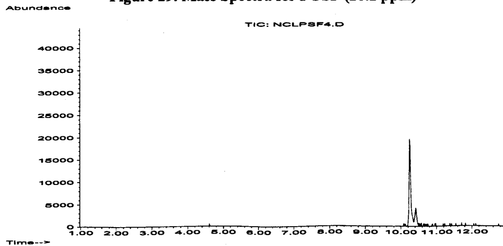
Figure 30. Total Ion Chromatogram for POSF (14.1 ppm)
