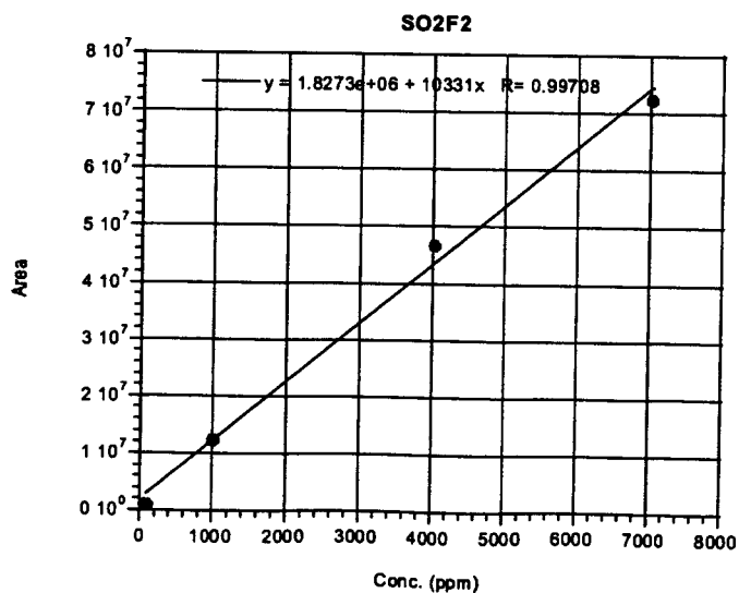
Figure 4. Calibration Plot for SO 2 F 2
