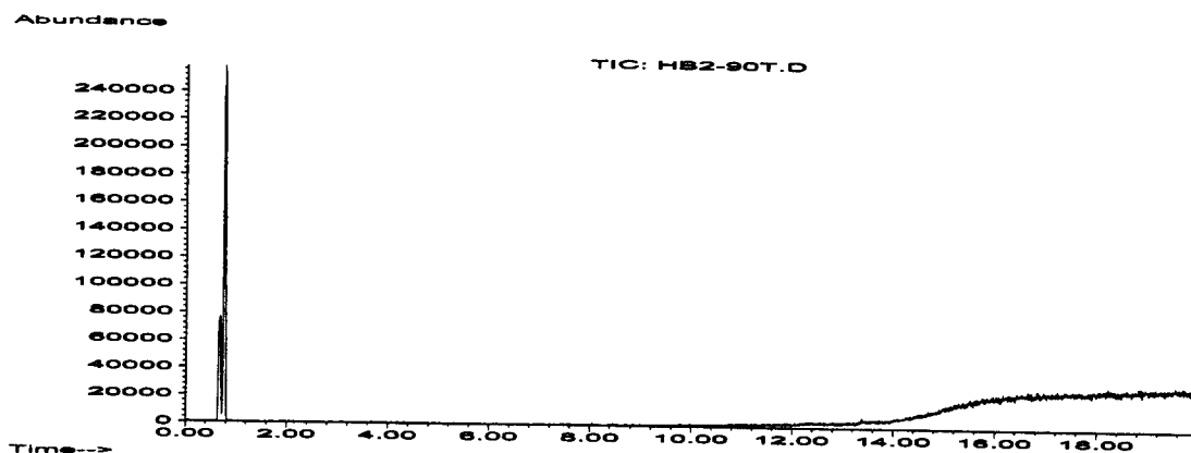
Figure 5.5.4. Off-line GC/MS Ion Chromatogram for Heated Blank at 900°C
