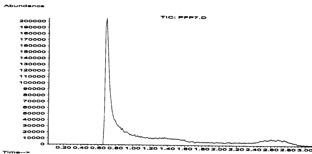
Figure 38. Total Ion Chromatogram for HFP (1,050 ppm)
