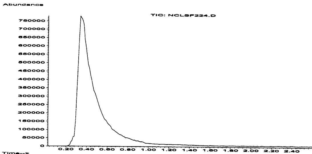
Figure 19. Total Ion Chromatogram for SO 2 F 2 (10049 ppm)
