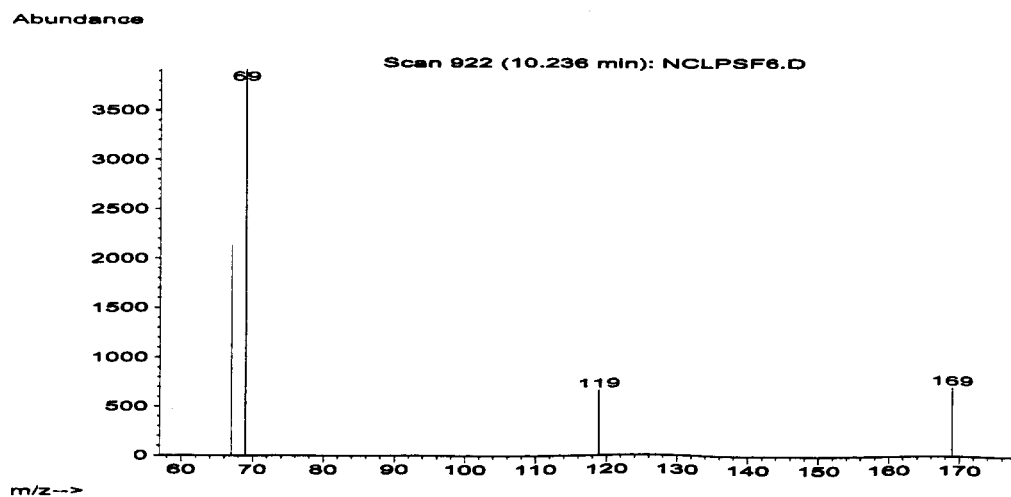
Figure 33. Mass Spectra for POSF (8.0 ppm)
