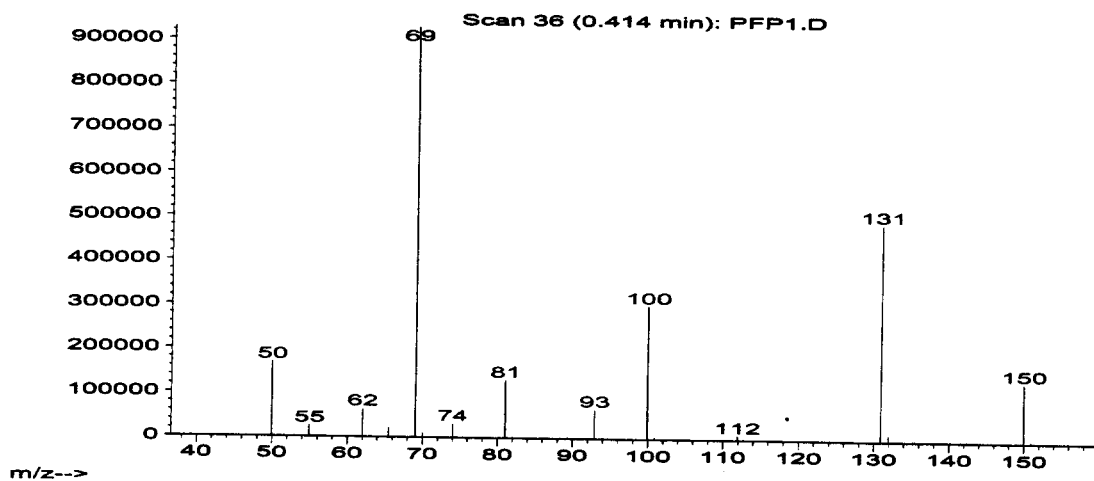
Figure 35. Mass Spectra for HFP (10,000 ppm)
