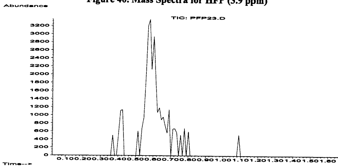
Figure 41. Total Ion Chromatogram for HFP (1.9 ppm)
