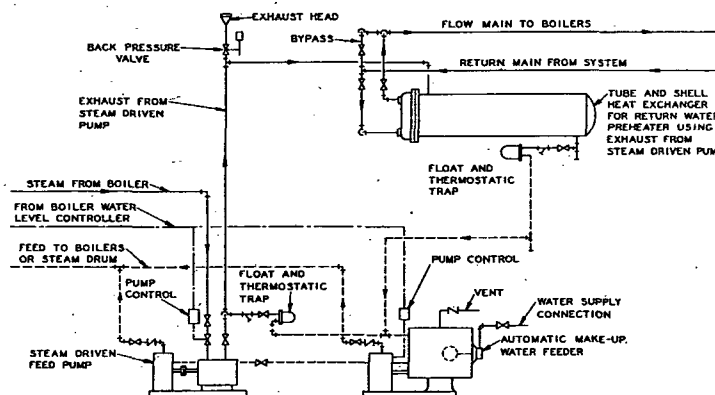
Fig. 15.... Arrangement of Boiler Feed Where Exhaust Steam Is Available
