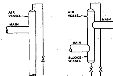
Fig. 14.... Methods of Venting High-Temperature Water Mains
